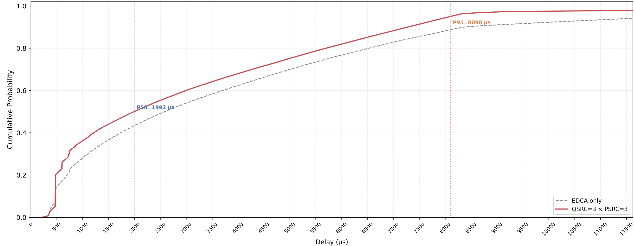
P-EDCA STA VO Delay CDF — QSRC=3 × PSRC=3 nSta=30, nPedca=30, 1Mbps, avg of 10 runs
