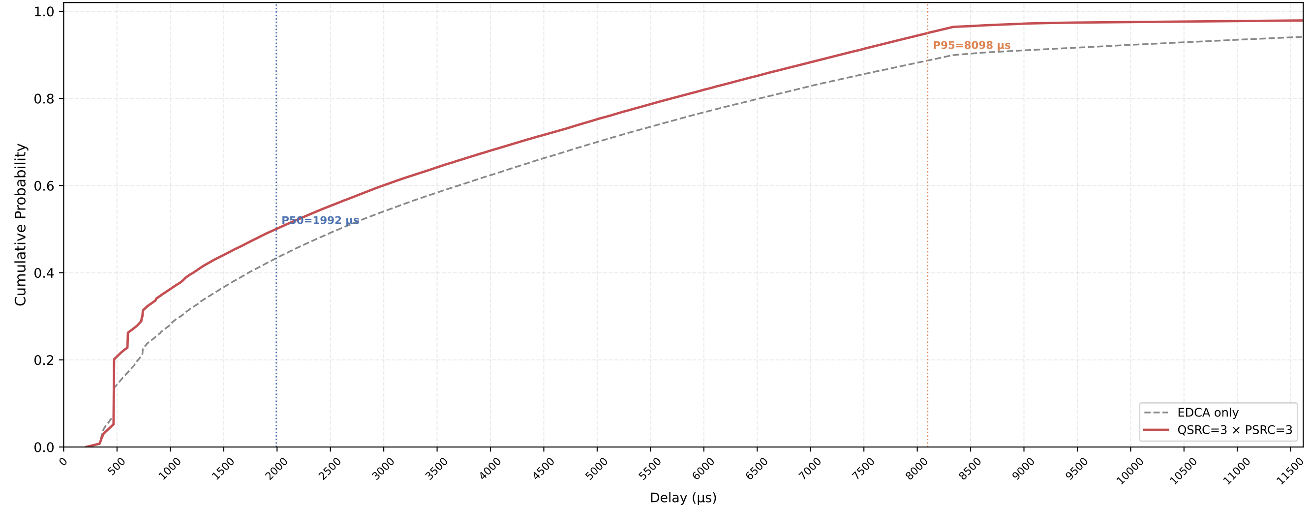
VO (all STAs) Delay CDF — QSRC=3 × PSRC=3 nSta=30, nPedca=30, 1Mbps, avg of 10 runs
