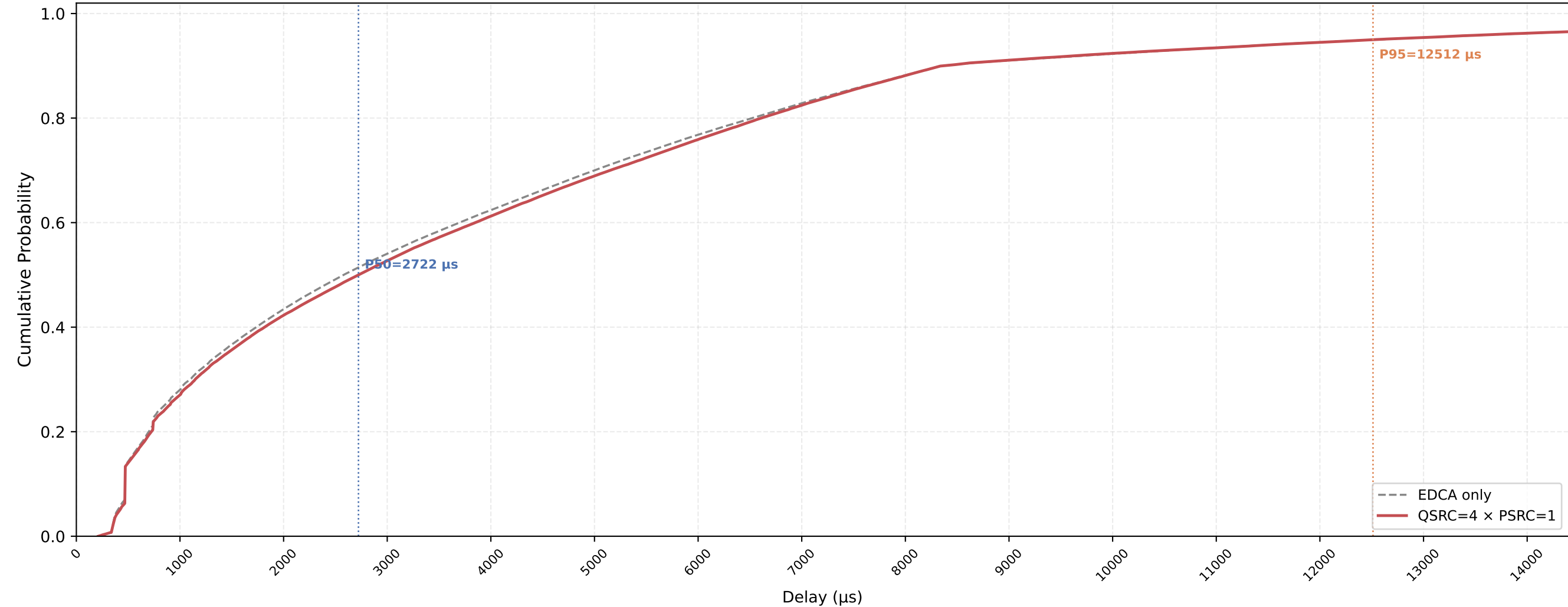
Legacy STA VO Delay CDF — QSRC=4 × PSRC=1 nSta=30, nPedca=15, 1Mbps, avg of 10 runs
