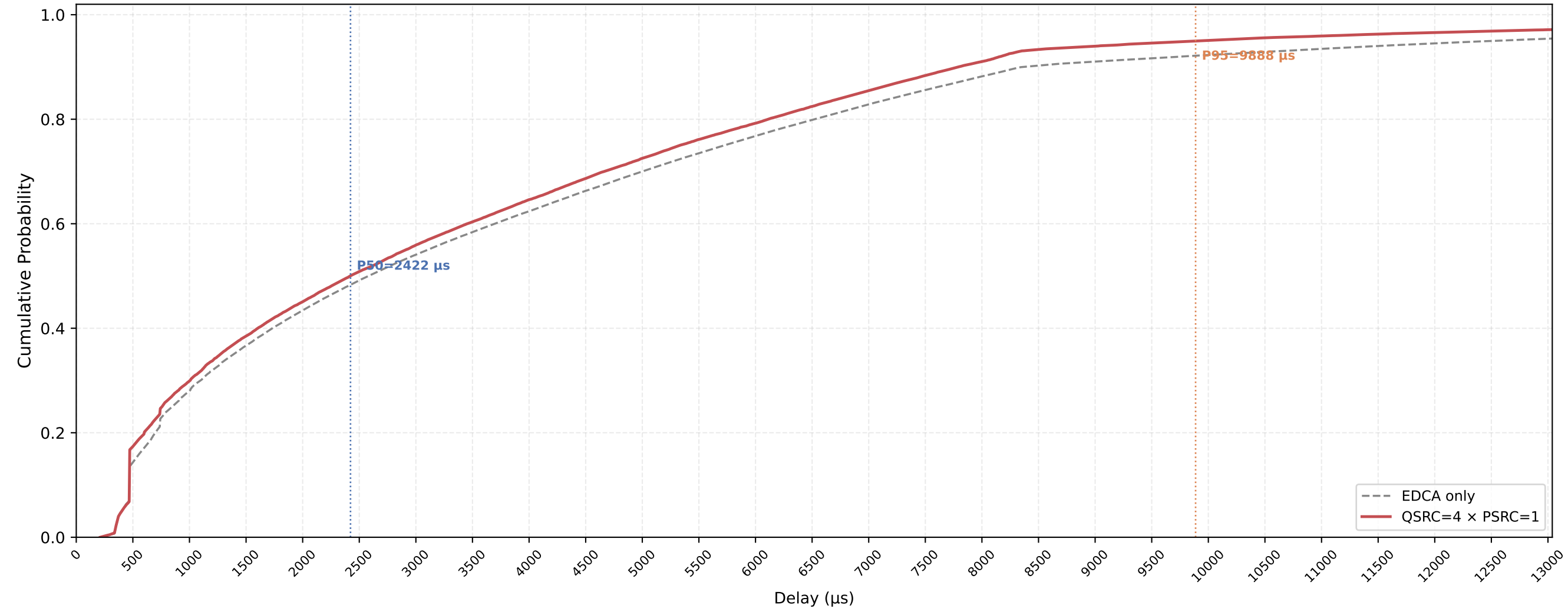
P-EDCA STA VO Delay CDF — QSRC=4 × PSRC=1 nSta=30, nPedca=5, 1Mbps, avg of 10 runs
