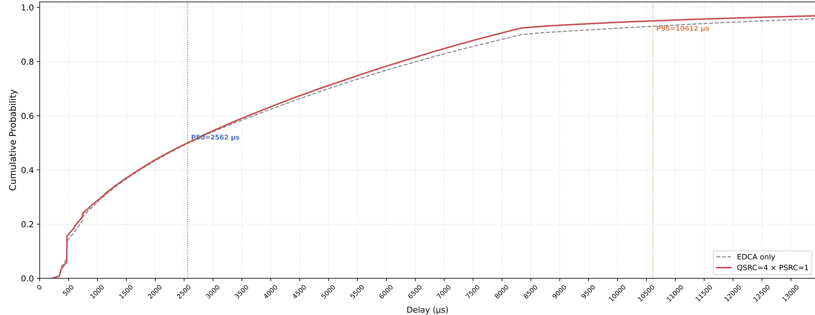
P-EDCA STA VO Delay CDF — QSRC=4 × PSRC=1 nSta=30, nPedca=30, 1Mbps, avg of 10 runs
