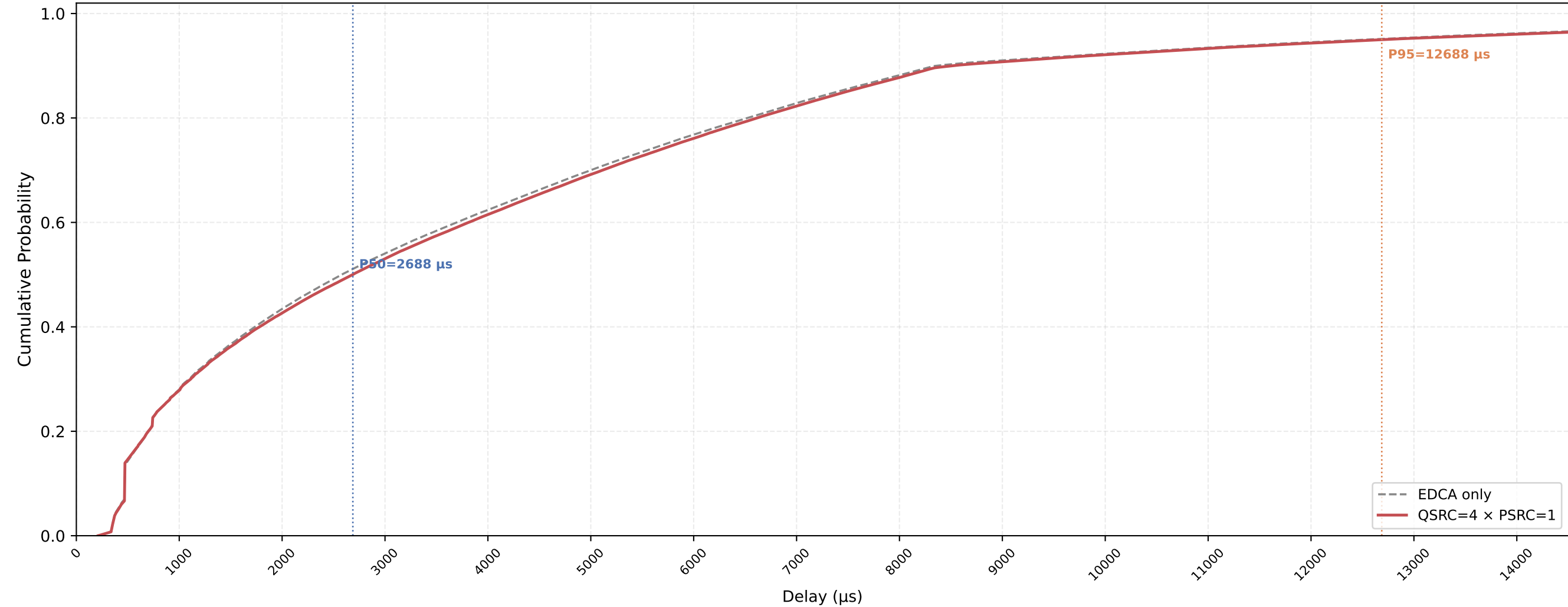
VO (all STAs) Delay CDF — QSRC=4 × PSRC=1 nSta=30, nPedca=5, 1Mbps, avg of 10 runs
