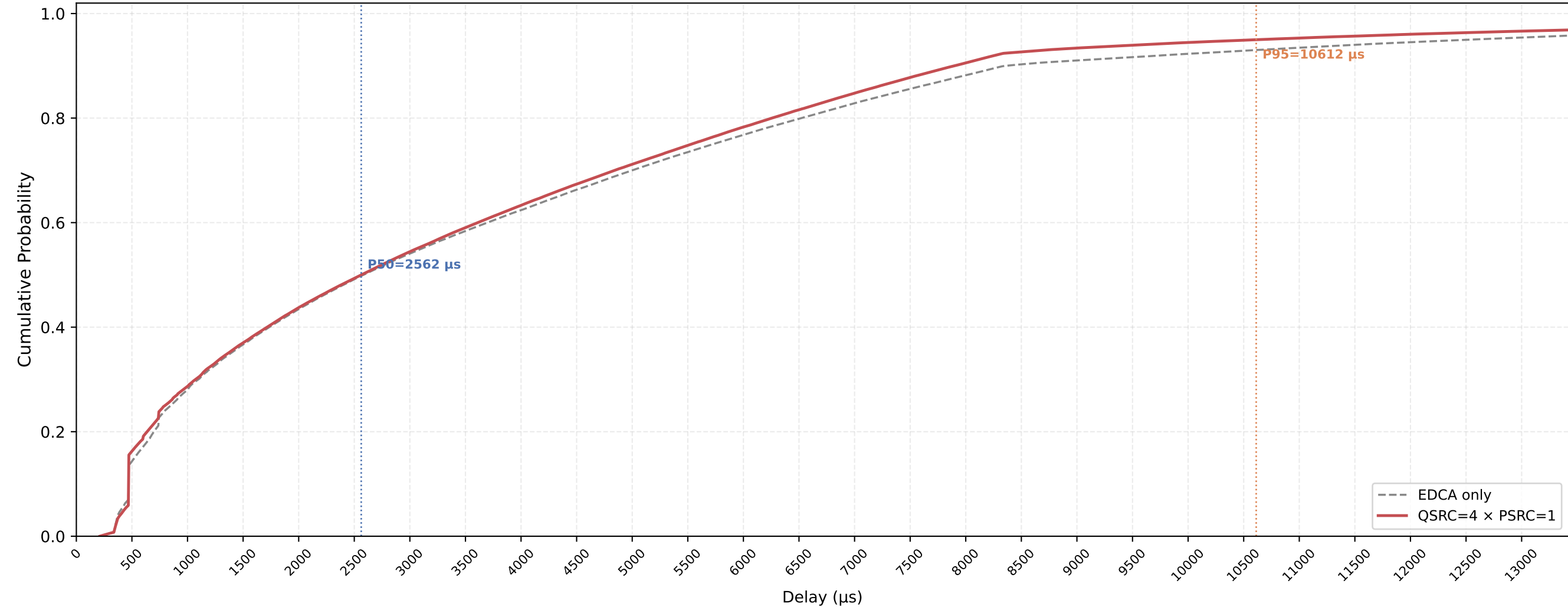
VO (all STAs) Delay CDF — QSRC=4 × PSRC=1 nSta=30, nPedca=30, 1Mbps, avg of 10 runs
