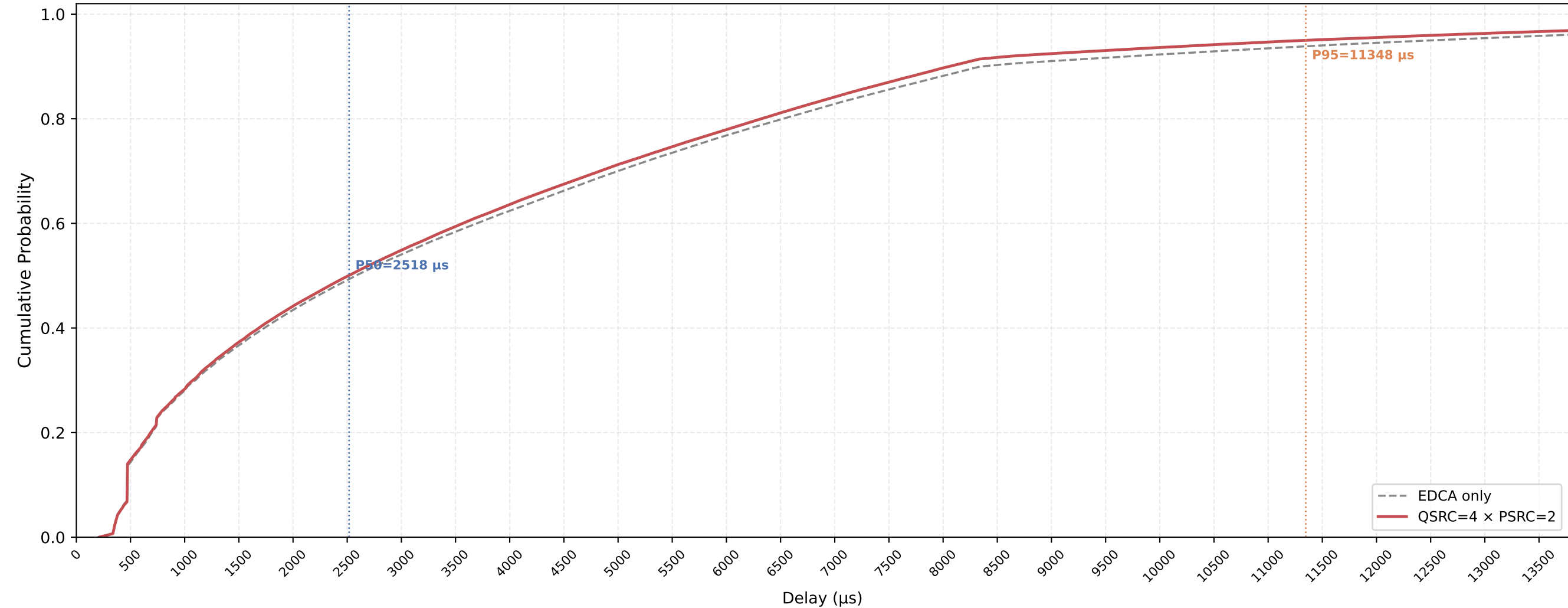
VO (all STAs) Delay CDF — QSRC=4 × PSRC=2 nSta=30, nPedca=5, 1Mbps, avg of 10 runs
