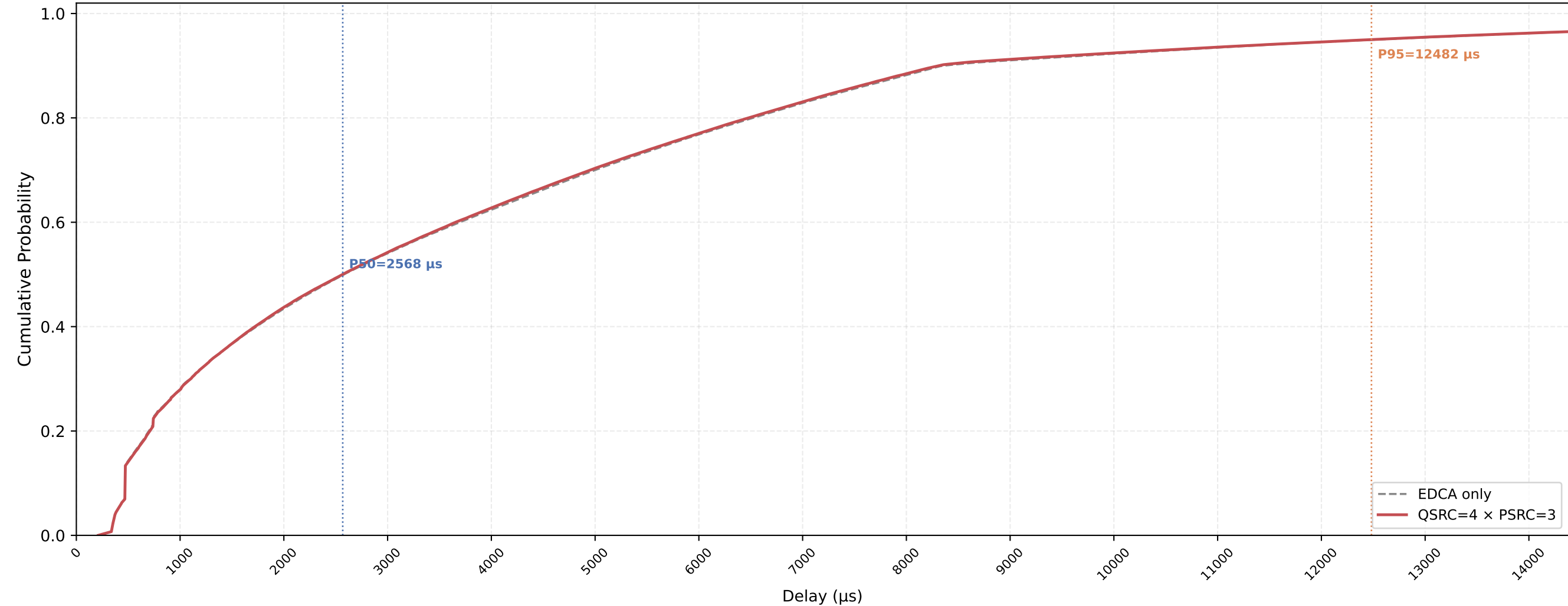
Legacy STA VO Delay CDF — QSRC=4 × PSRC=3 nSta=30, nPedca=5, 1Mbps, avg of 10 runs
