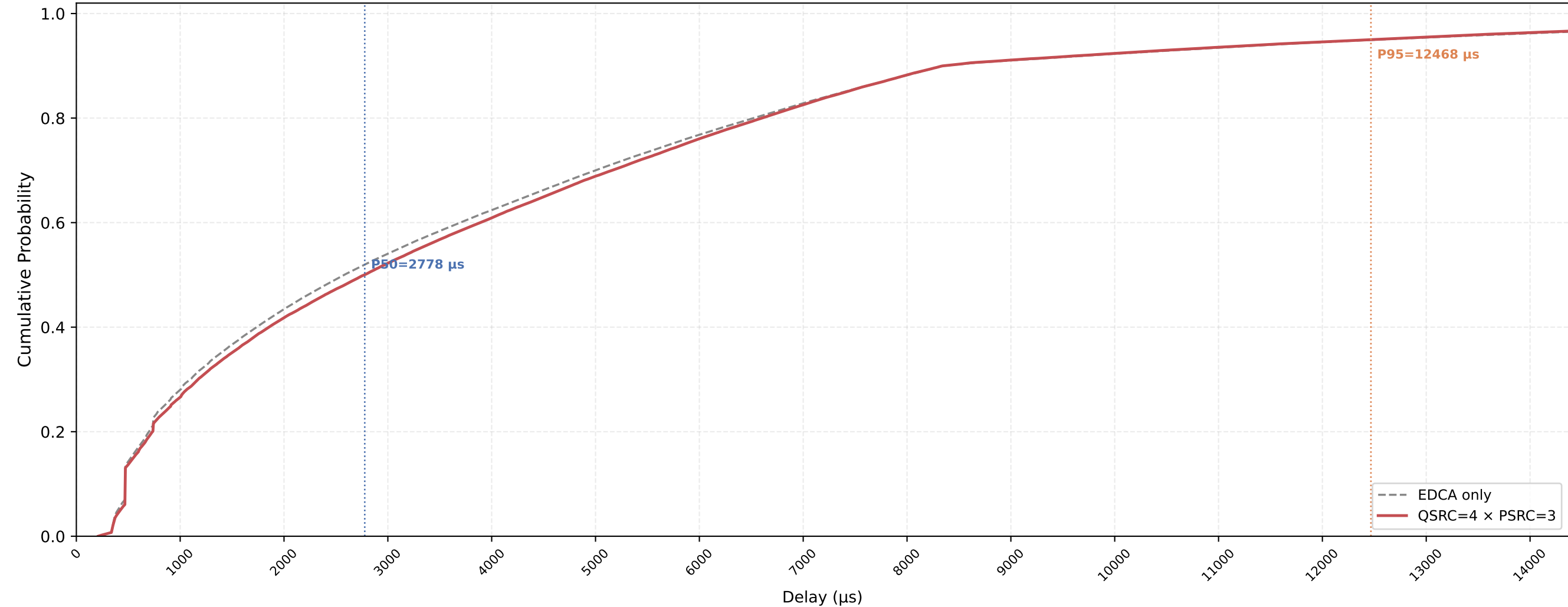
Legacy STA VO Delay CDF — QSRC=4 × PSRC=3 nSta=30, nPedca=15, 1Mbps, avg of 10 runs
