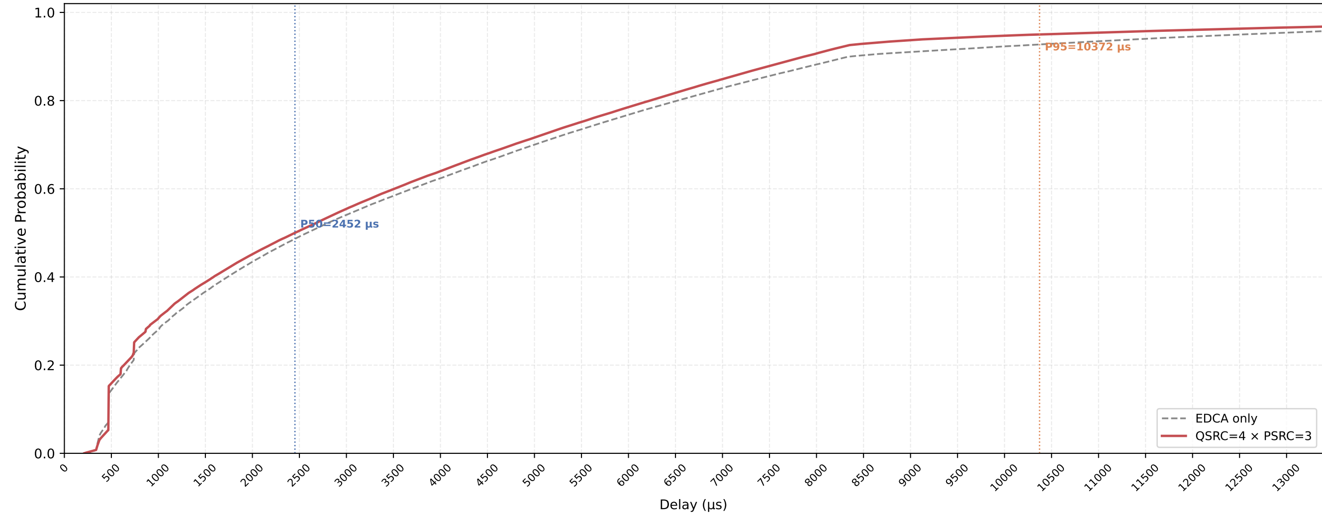
P-EDCA STA VO Delay CDF — QSRC=4 × PSRC=3 nSta=30, nPedca=30, 1Mbps, avg of 10 runs
