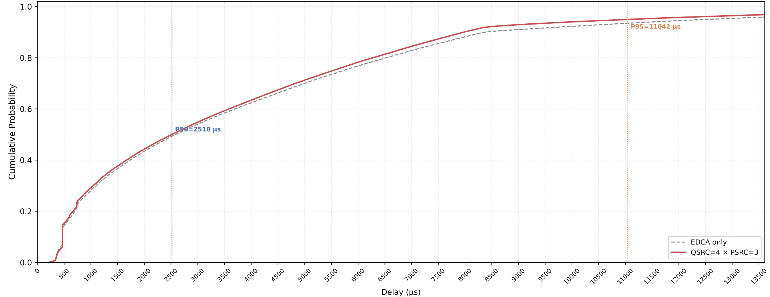
VO (all STAs) Delay CDF — QSRC=4 × PSRC=3 nSta=30, nPedca=15, 1Mbps, avg of 10 runs
