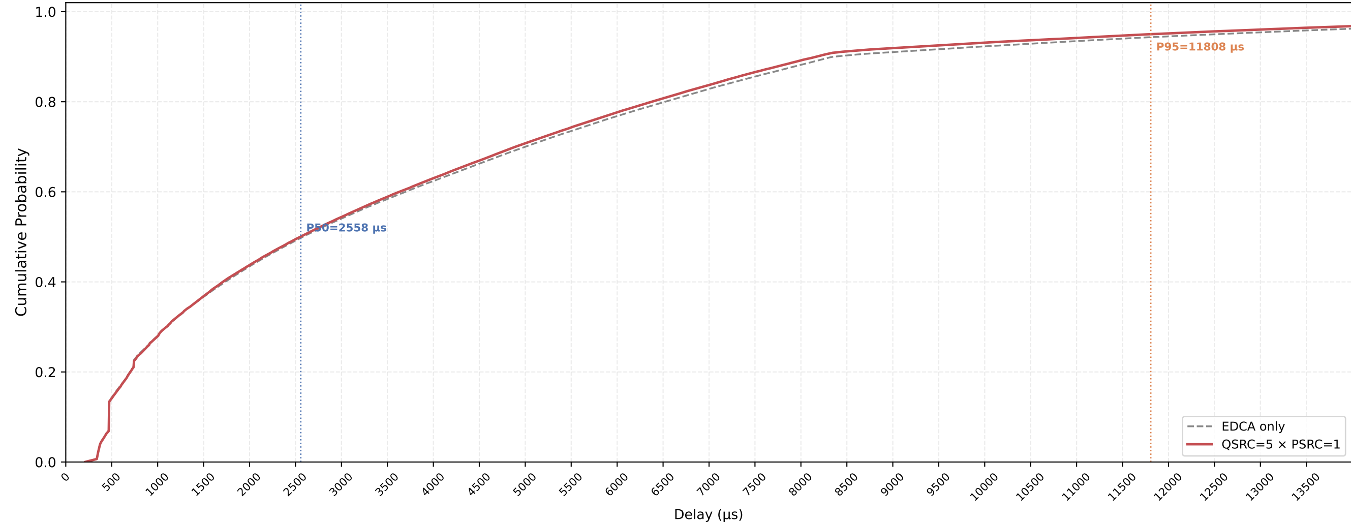
Legacy STA VO Delay CDF — QSRC=5 × PSRC=1 nSta=30, nPedca=5, 1Mbps, avg of 10 runs
