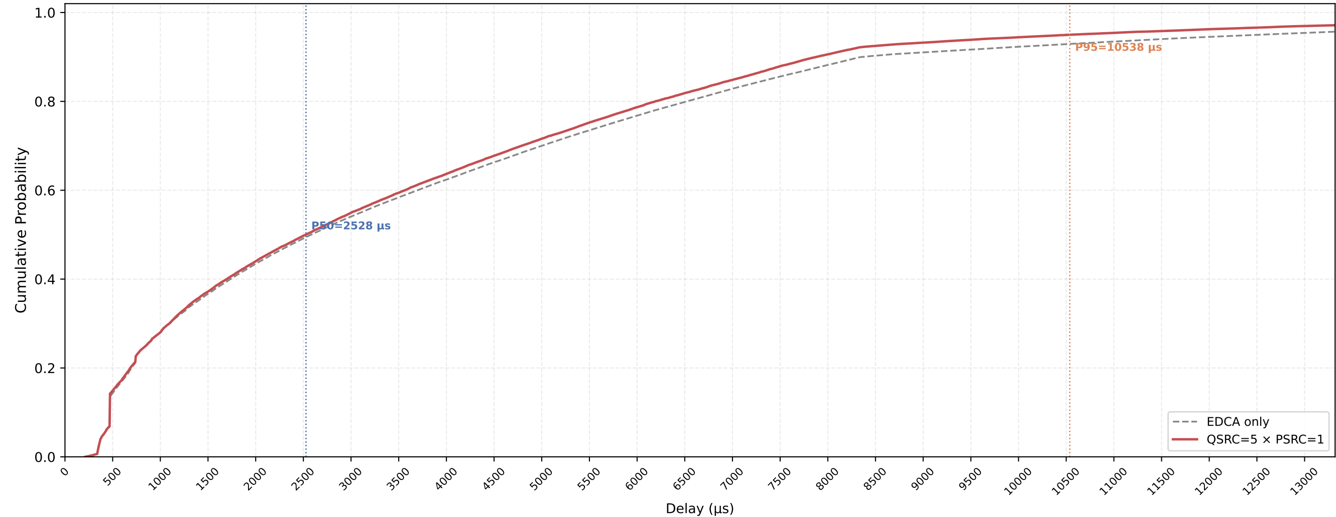
P-EDCA STA VO Delay CDF — QSRC=5 × PSRC=1 nSta=30, nPedca=5, 1Mbps, avg of 10 runs
