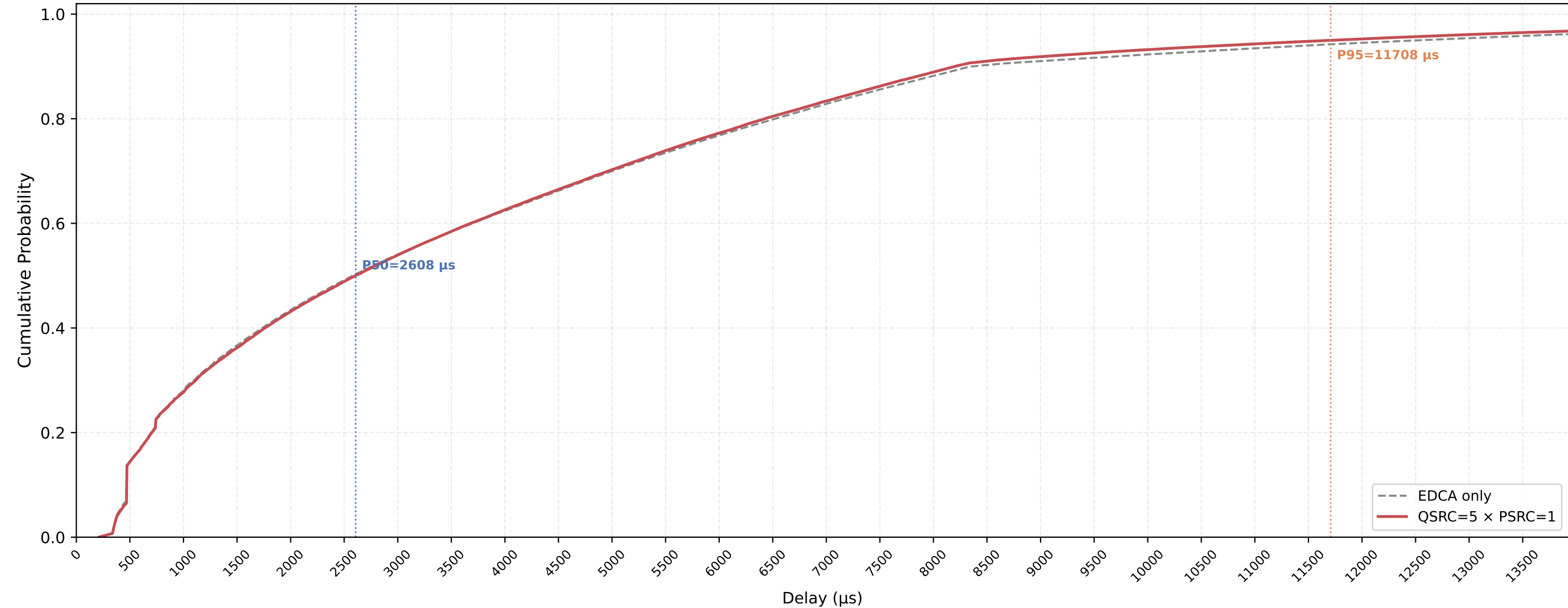
P-EDCA STA VO Delay CDF — QSRC=5 × PSRC=1 nSta=30, nPedca=15, 1Mbps, avg of 10 runs
