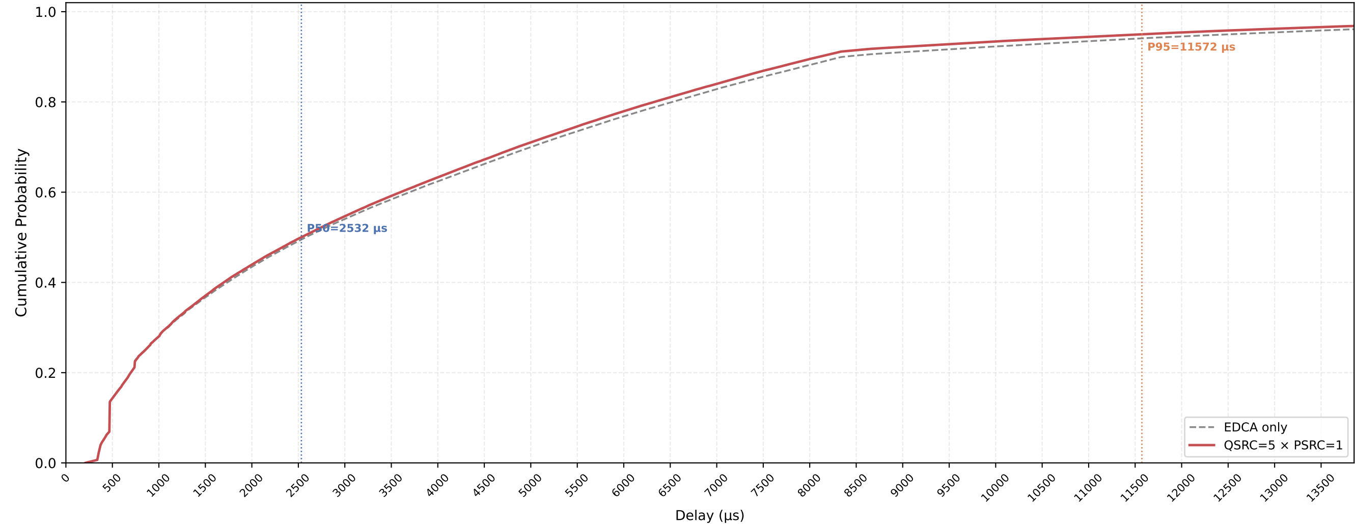
VO (all STAs) Delay CDF — QSRC=5 × PSRC=1 nSta=30, nPedca=5, 1Mbps, avg of 10 runs
