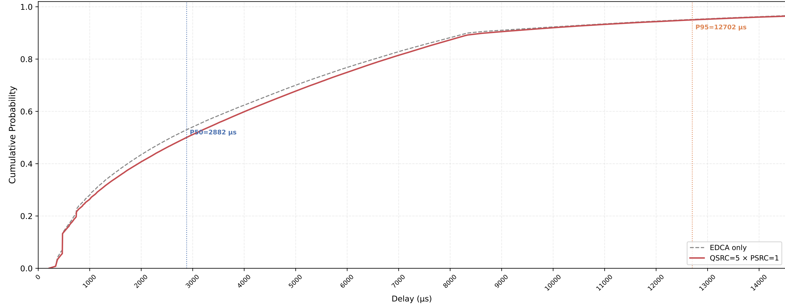
VO (all STAs) Delay CDF — QSRC=5 × PSRC=1 nSta=30, nPedca=30, 1Mbps, avg of 10 runs
