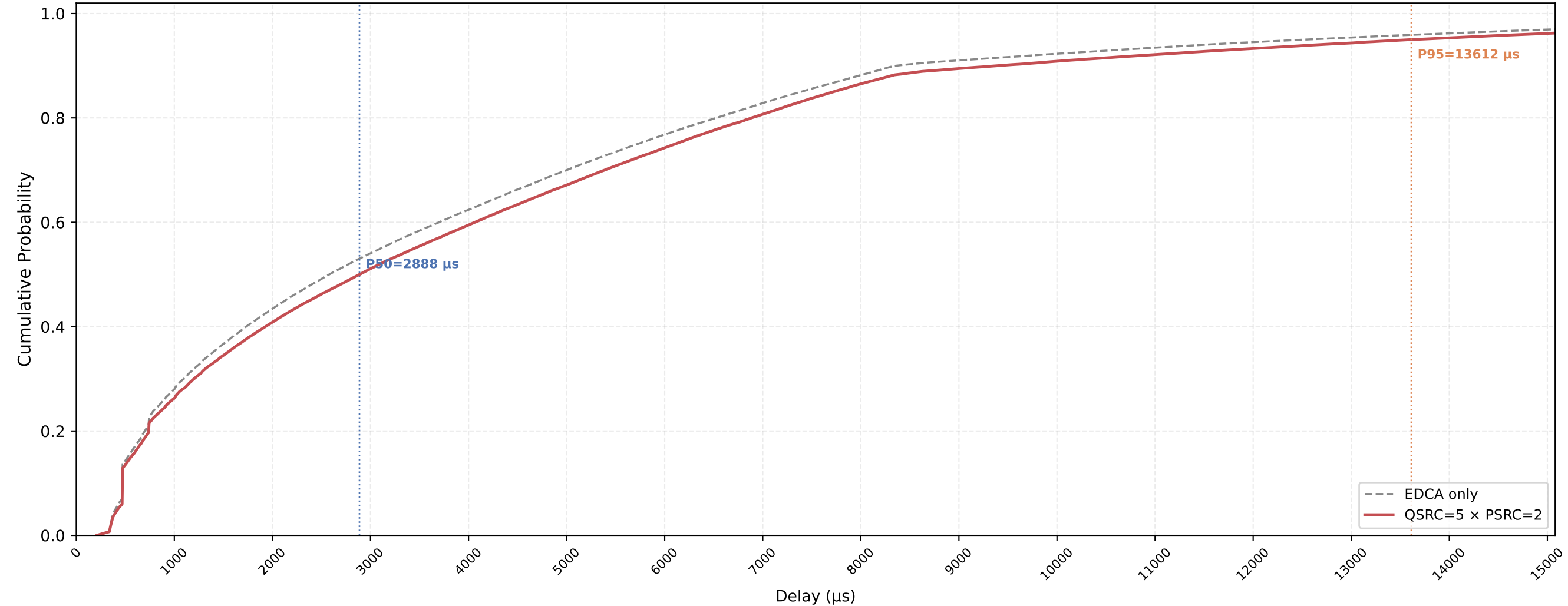
Legacy STA VO Delay CDF — QSRC=5 × PSRC=2 nSta=30, nPedca=15, 1Mbps, avg of 10 runs
