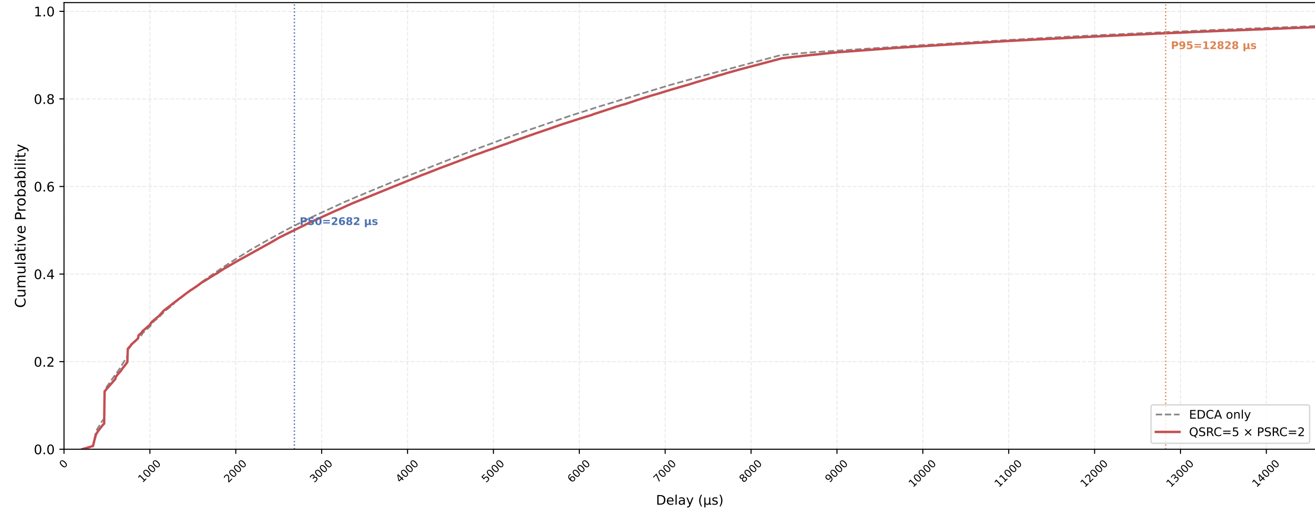
P-EDCA STA VO Delay CDF — QSRC=5 × PSRC=2 nSta=30, nPedca=15, 1Mbps, avg of 10 runs
