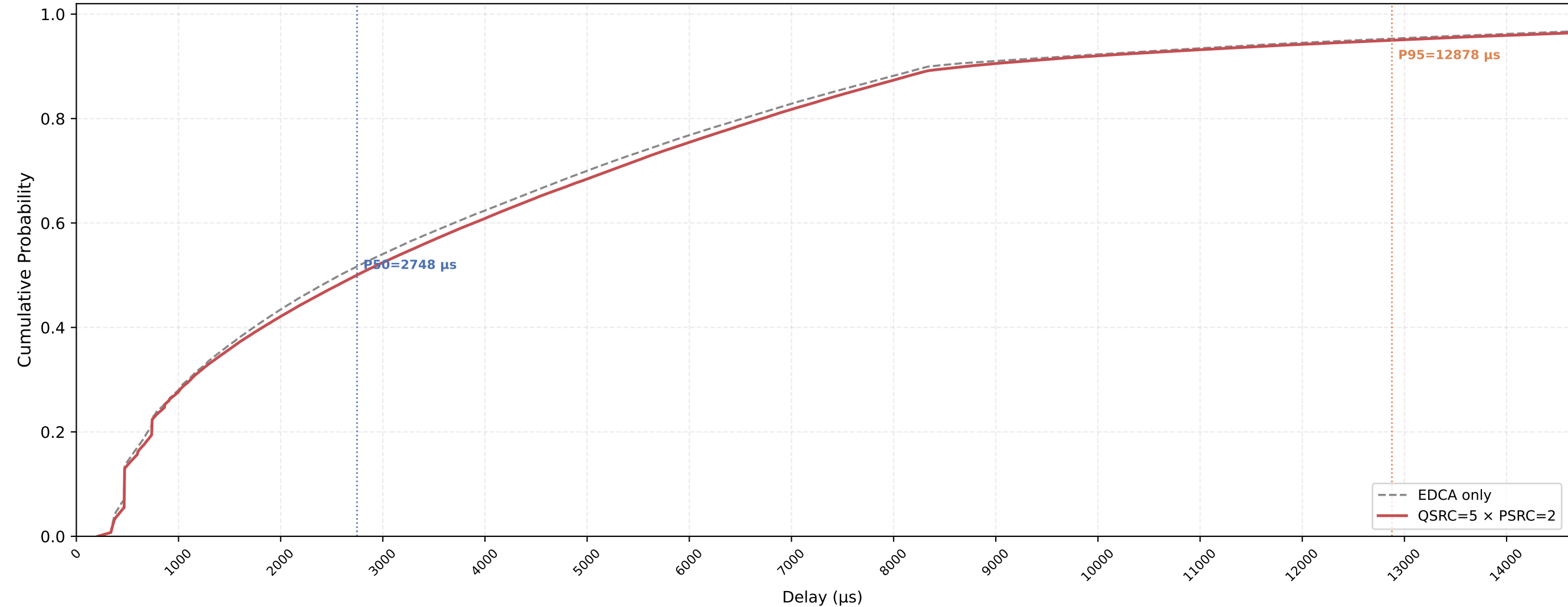
P-EDCA STA VO Delay CDF — QSRC=5 × PSRC=2 nSta=30, nPedca=30, 1Mbps, avg of 10 runs
