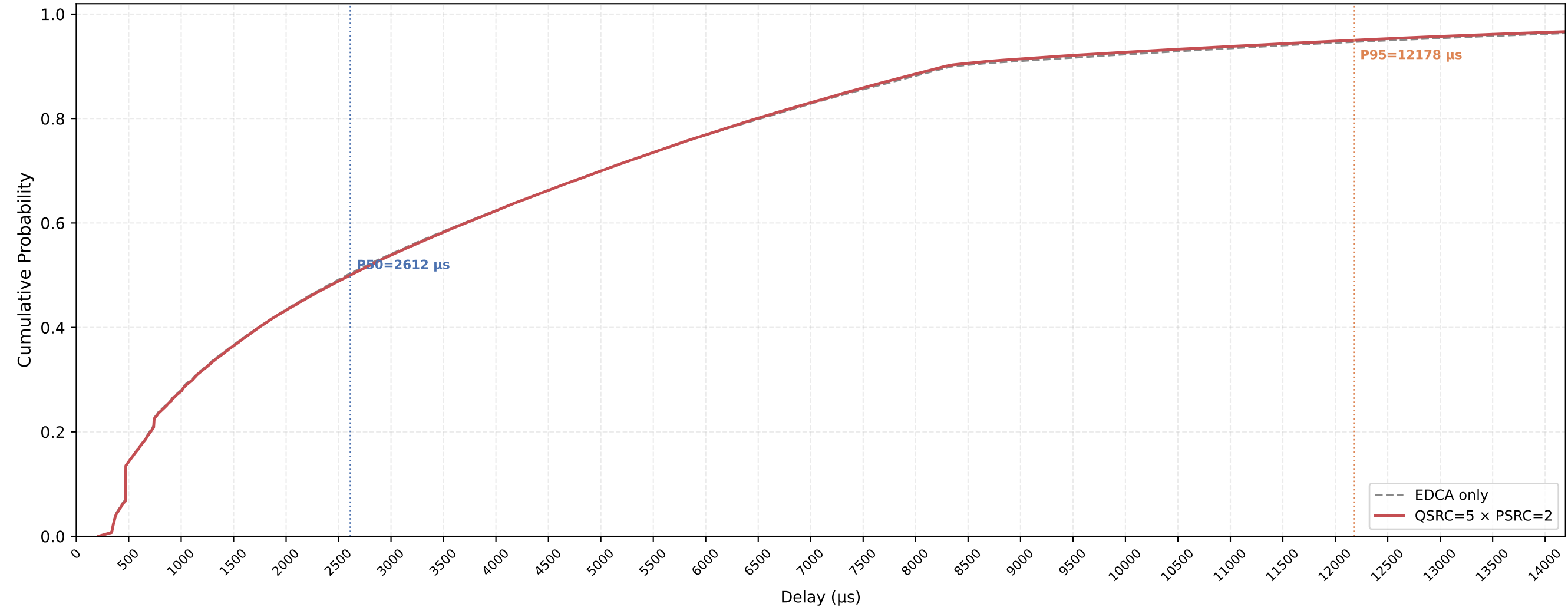
VO (all STAs) Delay CDF — QSRC=5 × PSRC=2 nSta=30, nPedca=5, 1Mbps, avg of 10 runs
