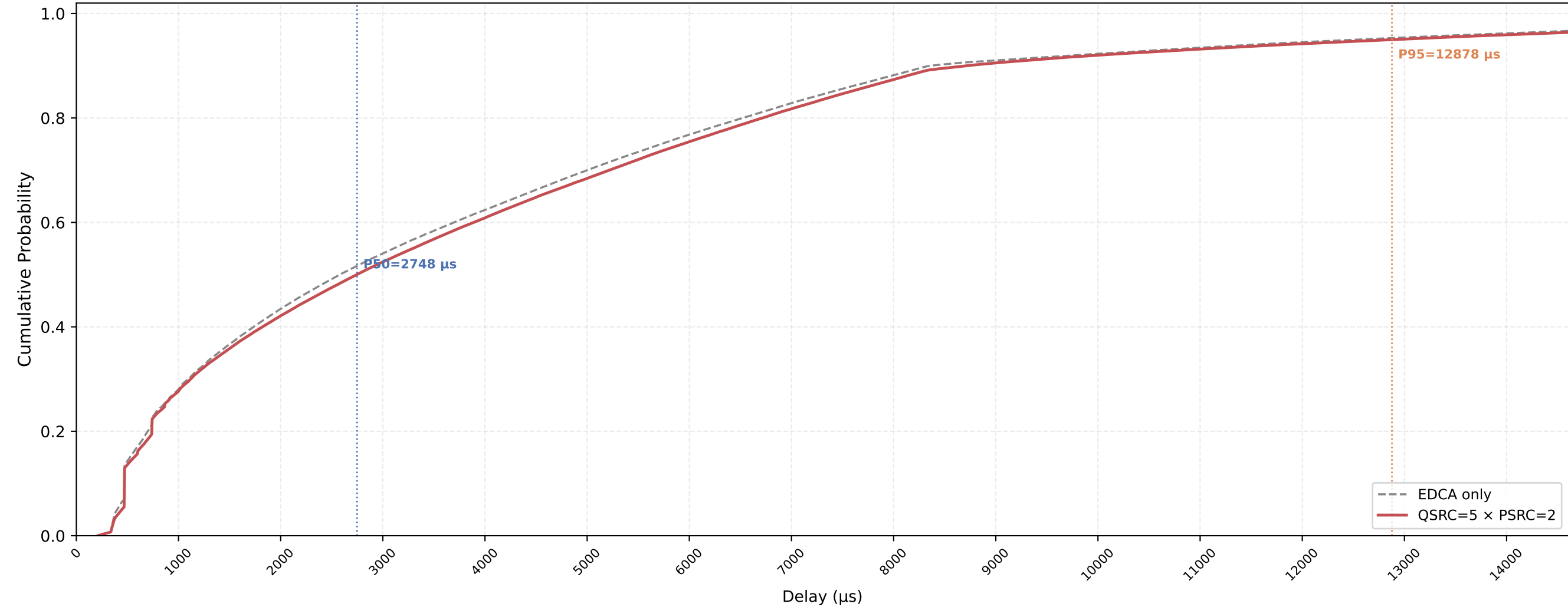
VO (all STAs) Delay CDF — QSRC=5 × PSRC=2 nSta=30, nPedca=30, 1Mbps, avg of 10 runs
