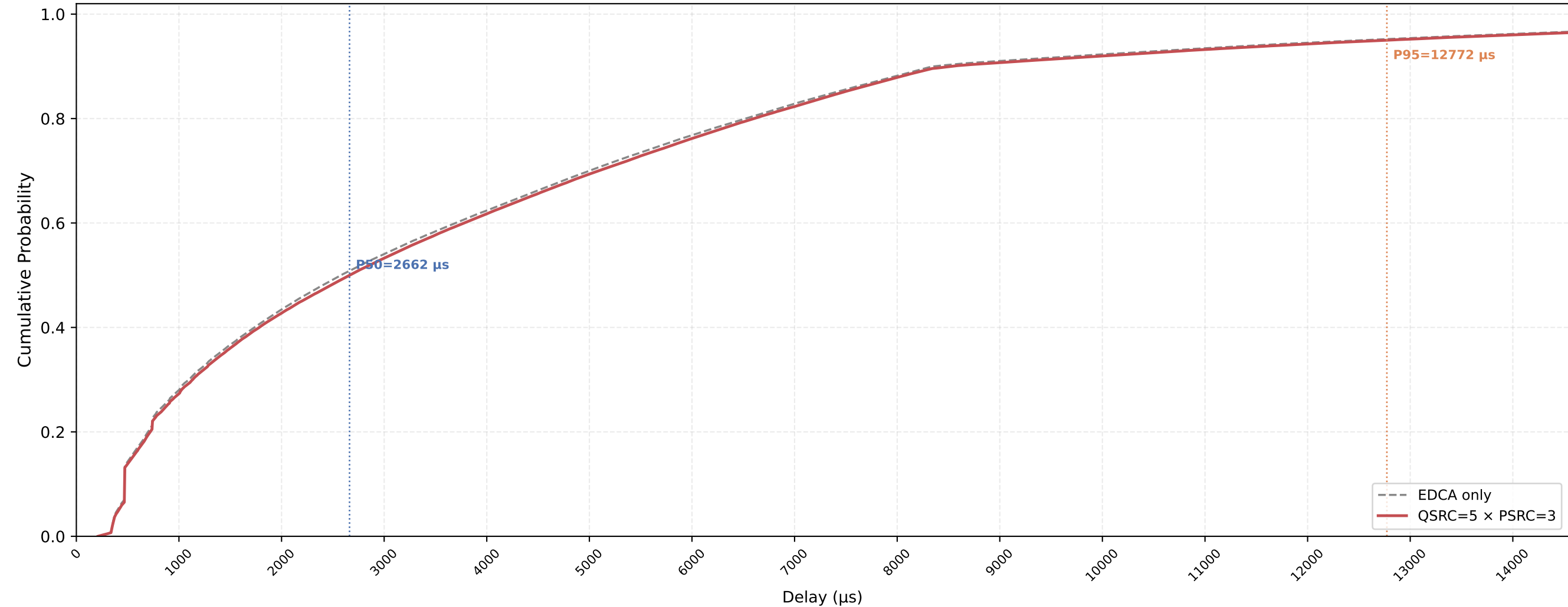
Legacy STA VO Delay CDF — QSRC=5 × PSRC=3 nSta=30, nPedca=5, 1Mbps, avg of 10 runs
