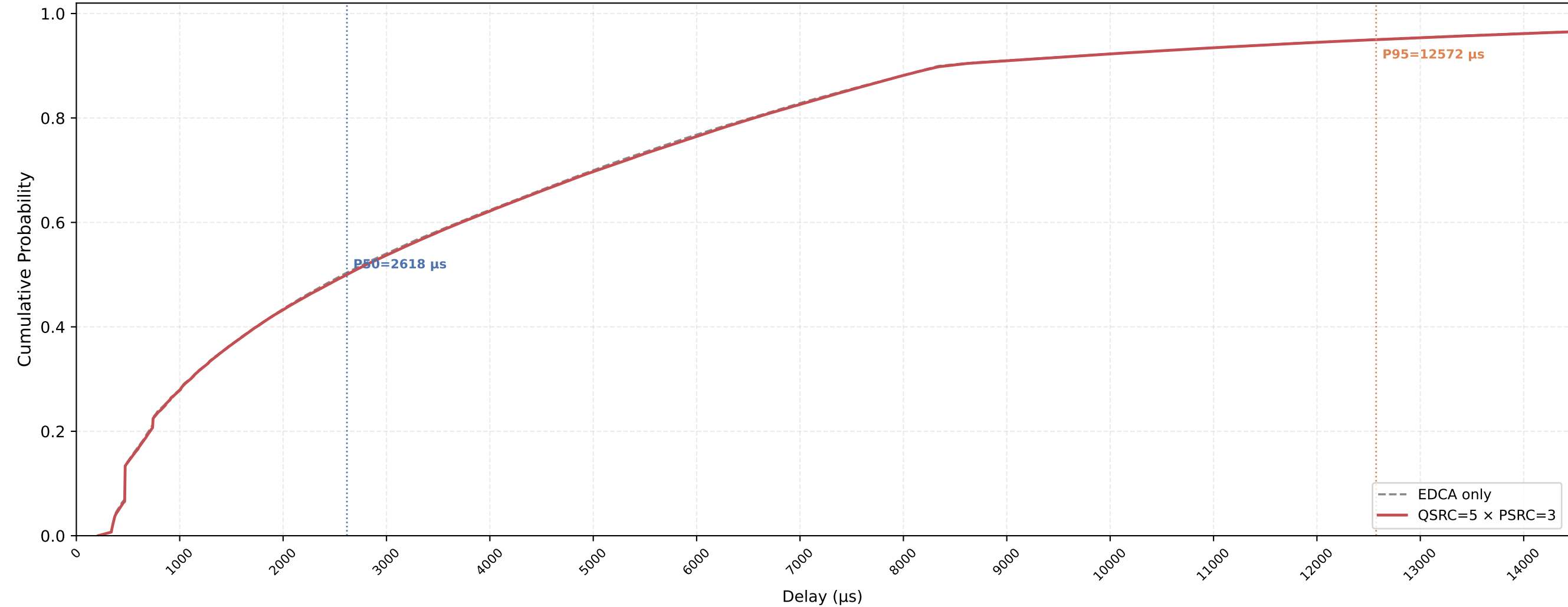
VO (all STAs) Delay CDF — QSRC=5 × PSRC=3 nSta=30, nPedca=5, 1Mbps, avg of 10 runs
