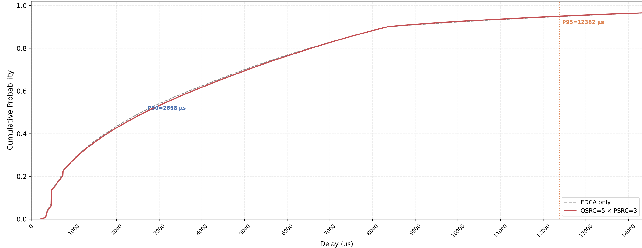
VO (all STAs) Delay CDF — QSRC=5 × PSRC=3 nSta=30, nPedca=15, 1Mbps, avg of 10 runs
