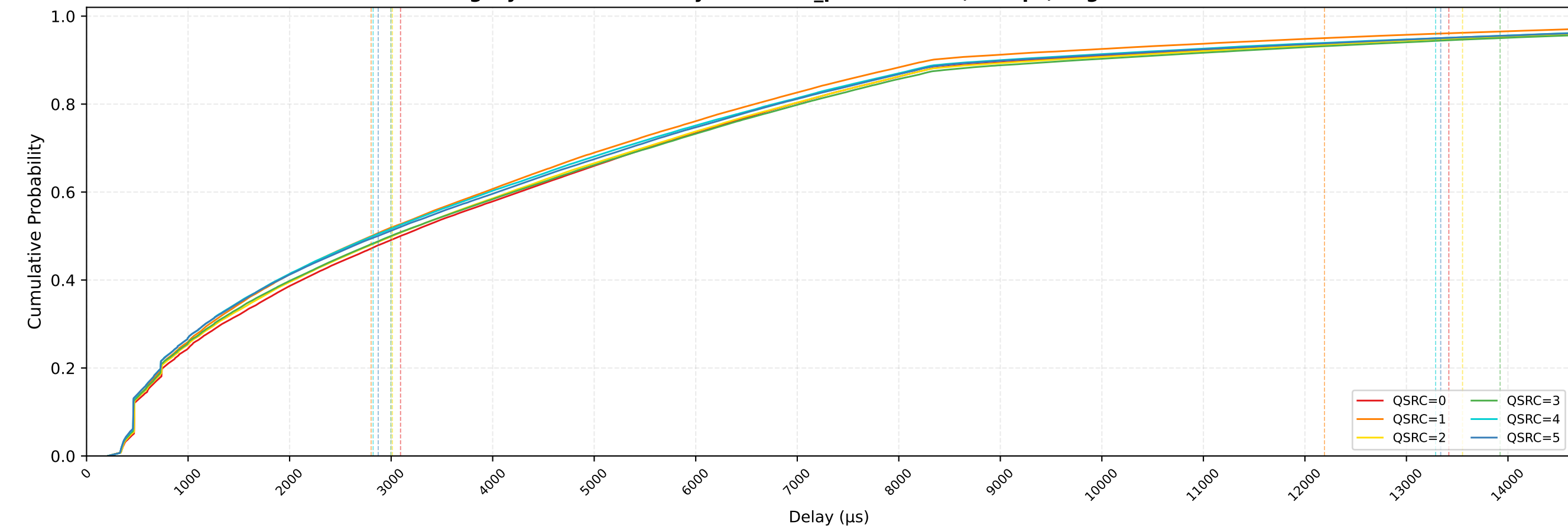
Legacy EDCA STAs Delay CDF — n_pedca=15/30, 1Mbps, avg of 10 runs
