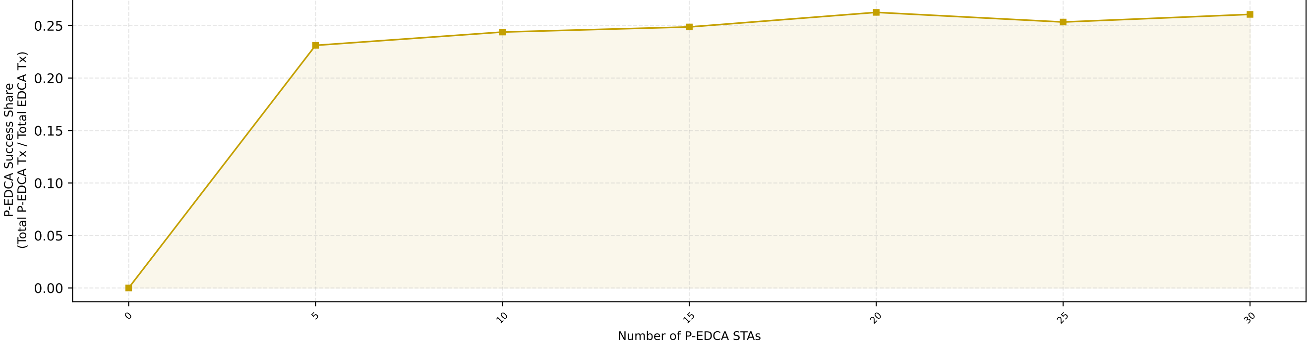
P-EDCA Tx / Total EDCA Tx — nSta=30, 1Mbps (avg of 10 runs)
