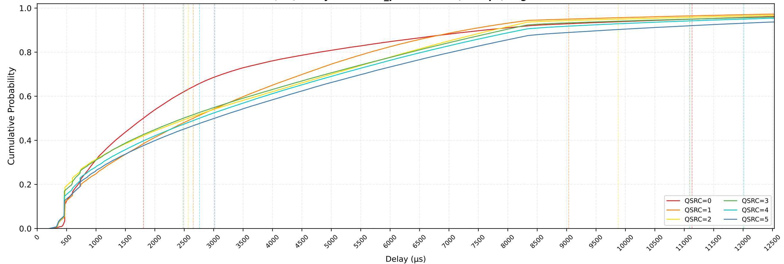
All STAs (VO) Delay CDF — n_pedca=25/30, 1Mbps, avg of 10 runs
