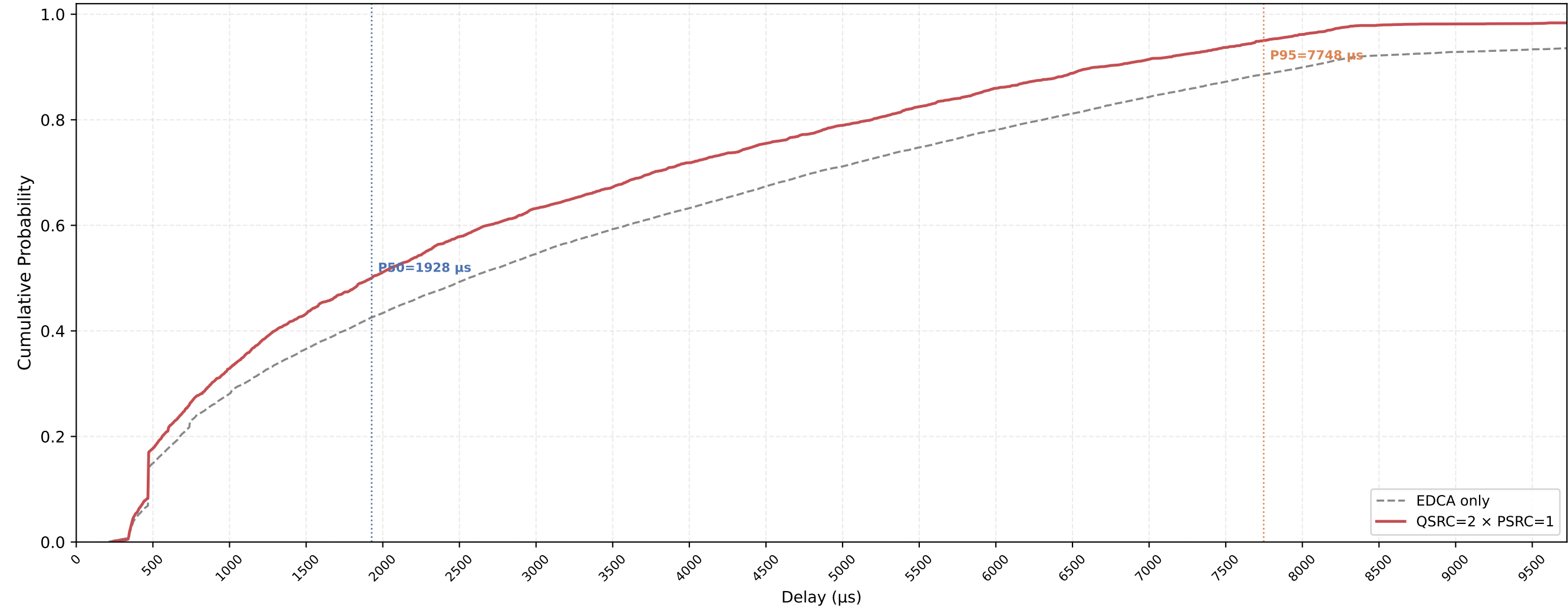
P-EDCA STA VO Delay CDF — QSRC=2 × PSRC=1 nSta=30, nPedca=5, 1Mbps
