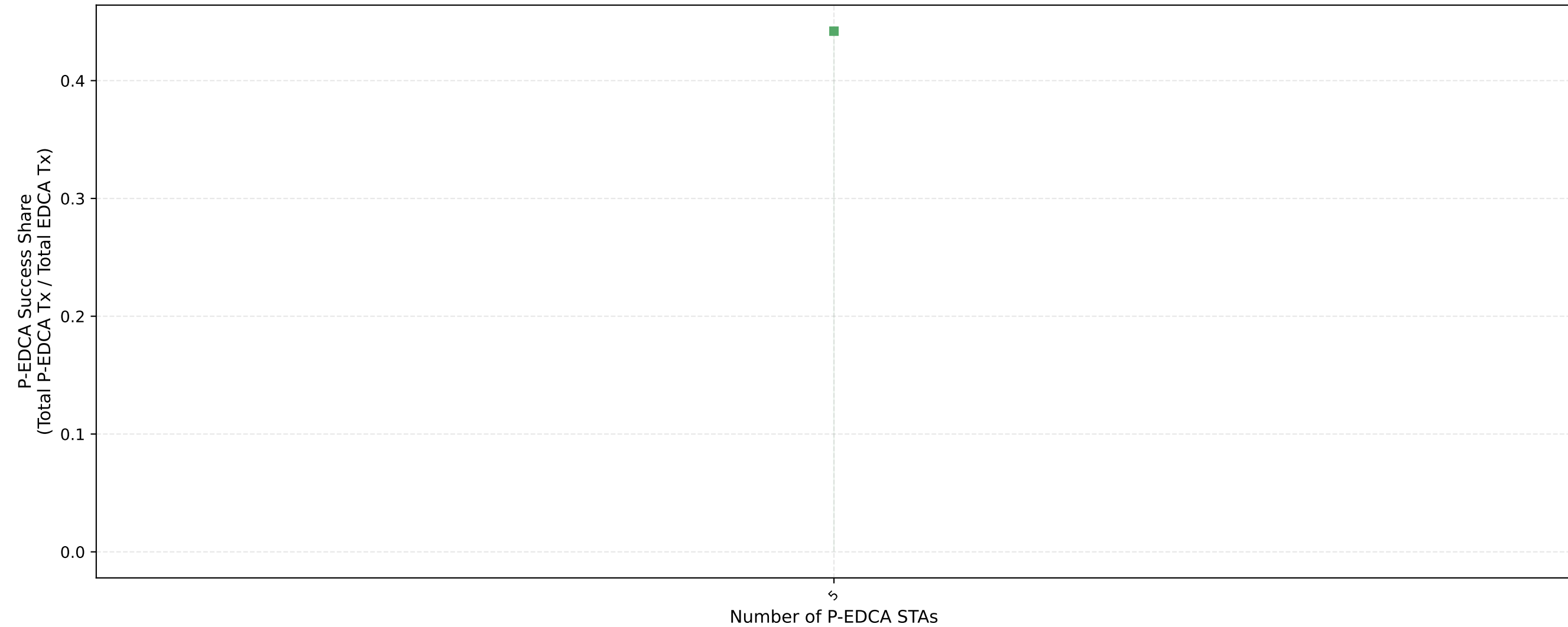
P-EDCA Tx / Total EDCA Tx — nSta=30, 1Mbps
