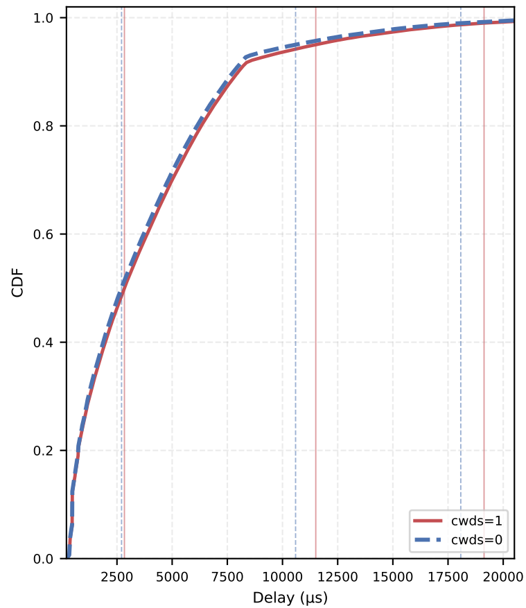
VO Delay CDF: cwds=0 vs cwds=1 | QSRC=2, PSRC=1, nSta=30, 1Mbps, avg of 10 runs
