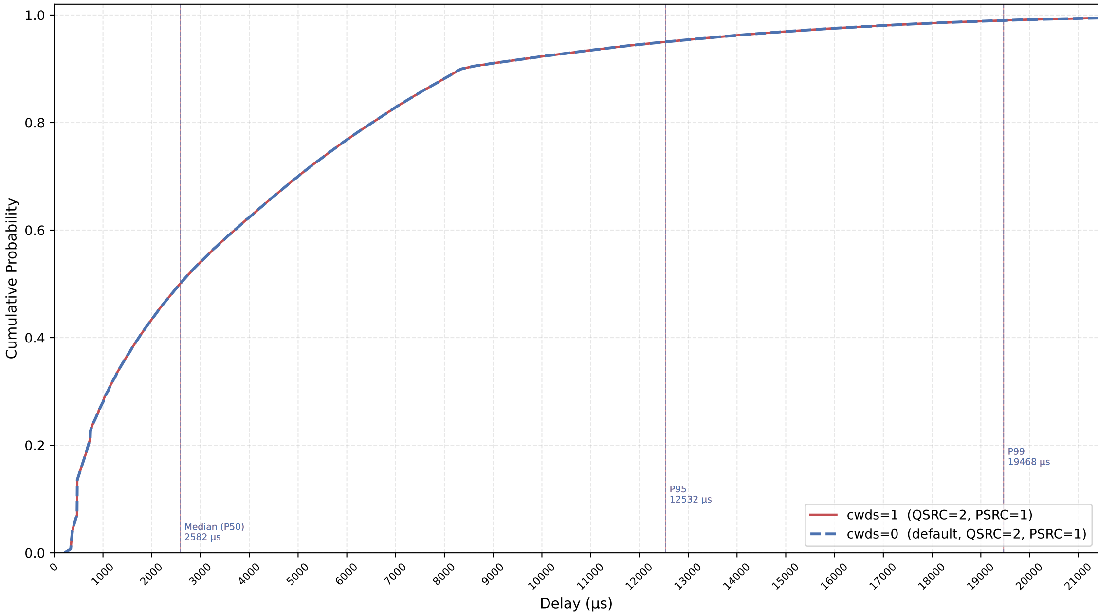
VO Delay CDF: cwds=0 vs cwds=1 — nSta=30, nPedca=0, QSRC=2, PSRC=1, 1Mbps, avg of 10 runs
