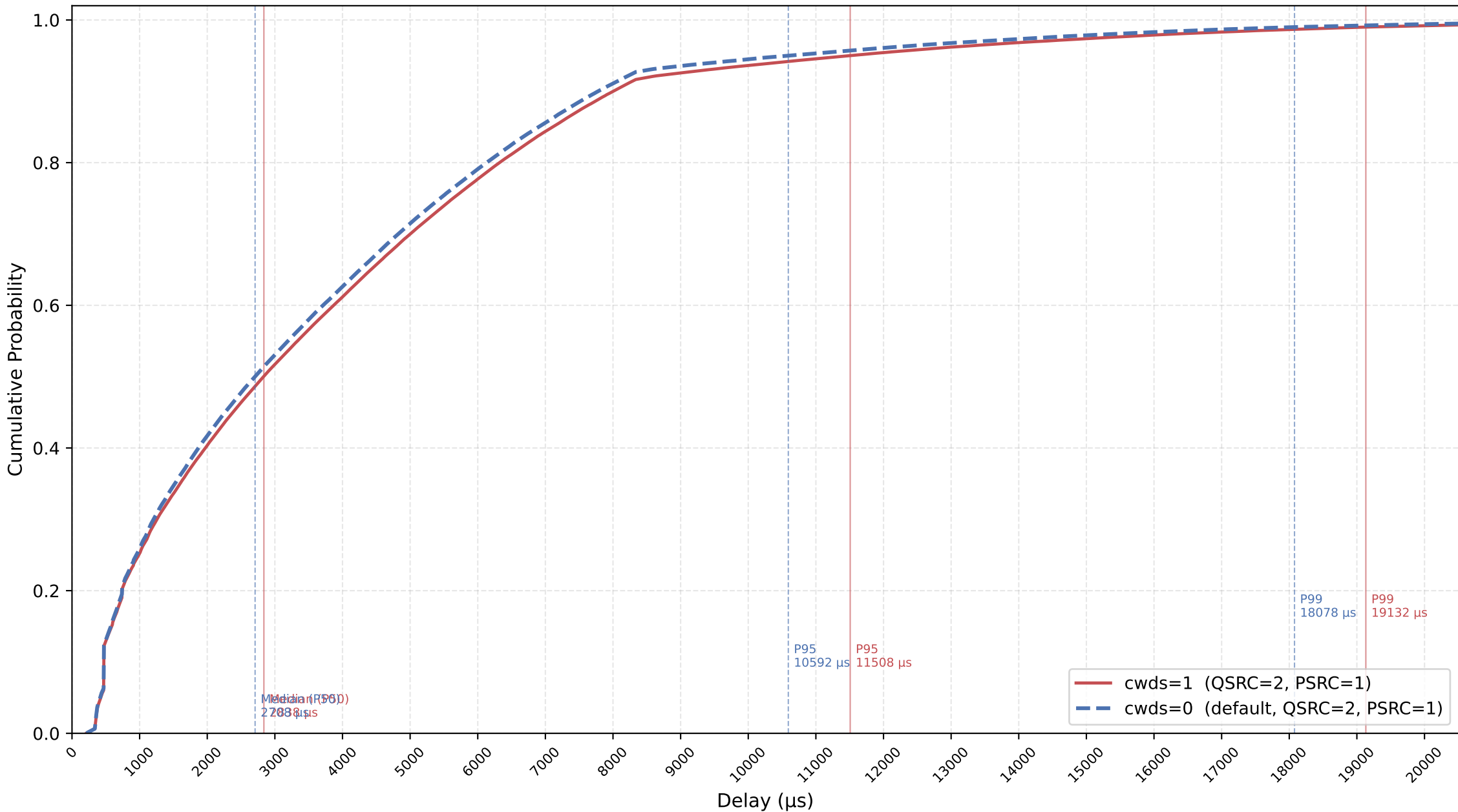
VO Delay CDF: cwds=0 vs cwds=1 — nSta=30, nPedca=10, QSRC=2, PSRC=1, 1Mbps, avg of 10 runs
