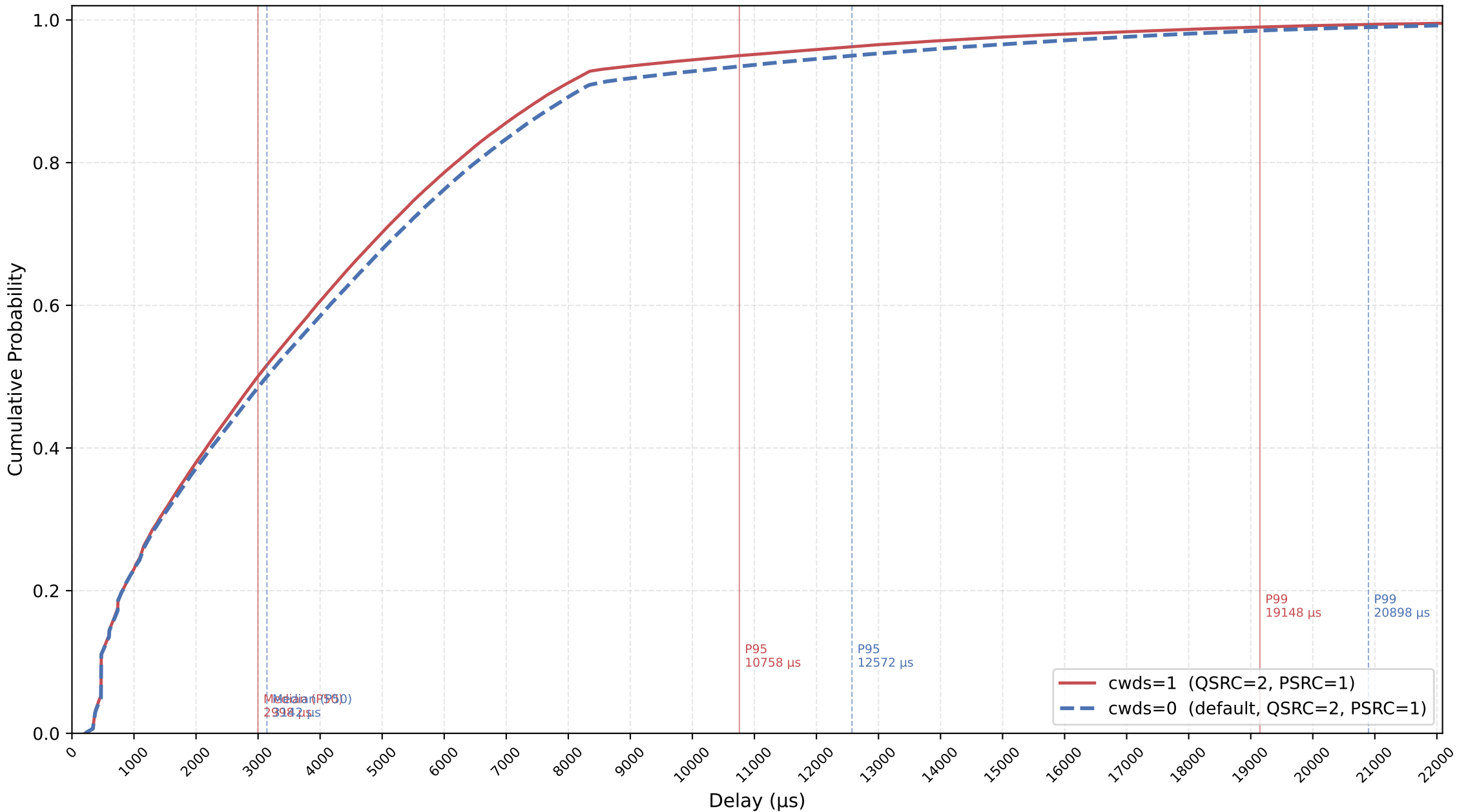
VO Delay CDF: cwds=0 vs cwds=1 — nSta=30, nPedca=25, QSRC=2, PSRC=1, 1Mbps, avg of 10 runs
