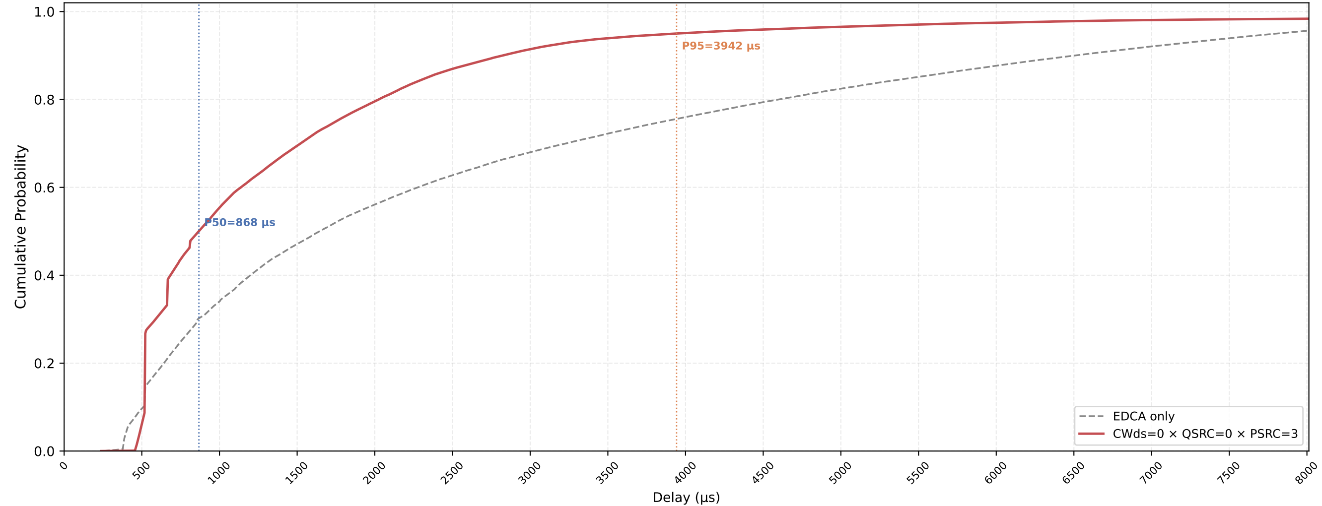
P-EDCA STA VO Delay CDF — CWds=0 × QSRC=0 × PSRC=3 nSta=30, nPedca=30, 1Mbps, avg of 10 runs
