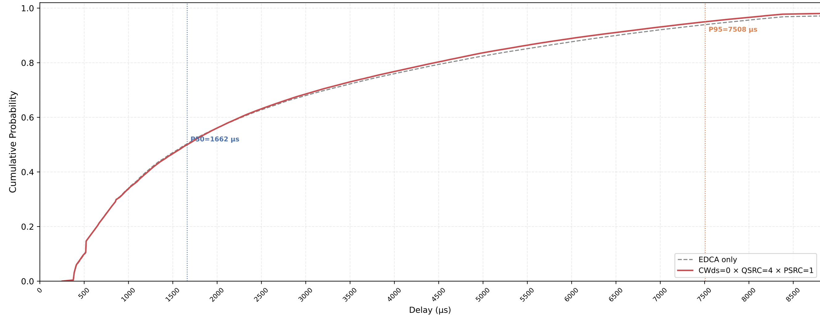
VO (all STAs) Delay CDF — CWds=0 × QSRC=4 × PSRC=1 nSta=30, nPedca=5, 1Mbps, avg of 10 runs
