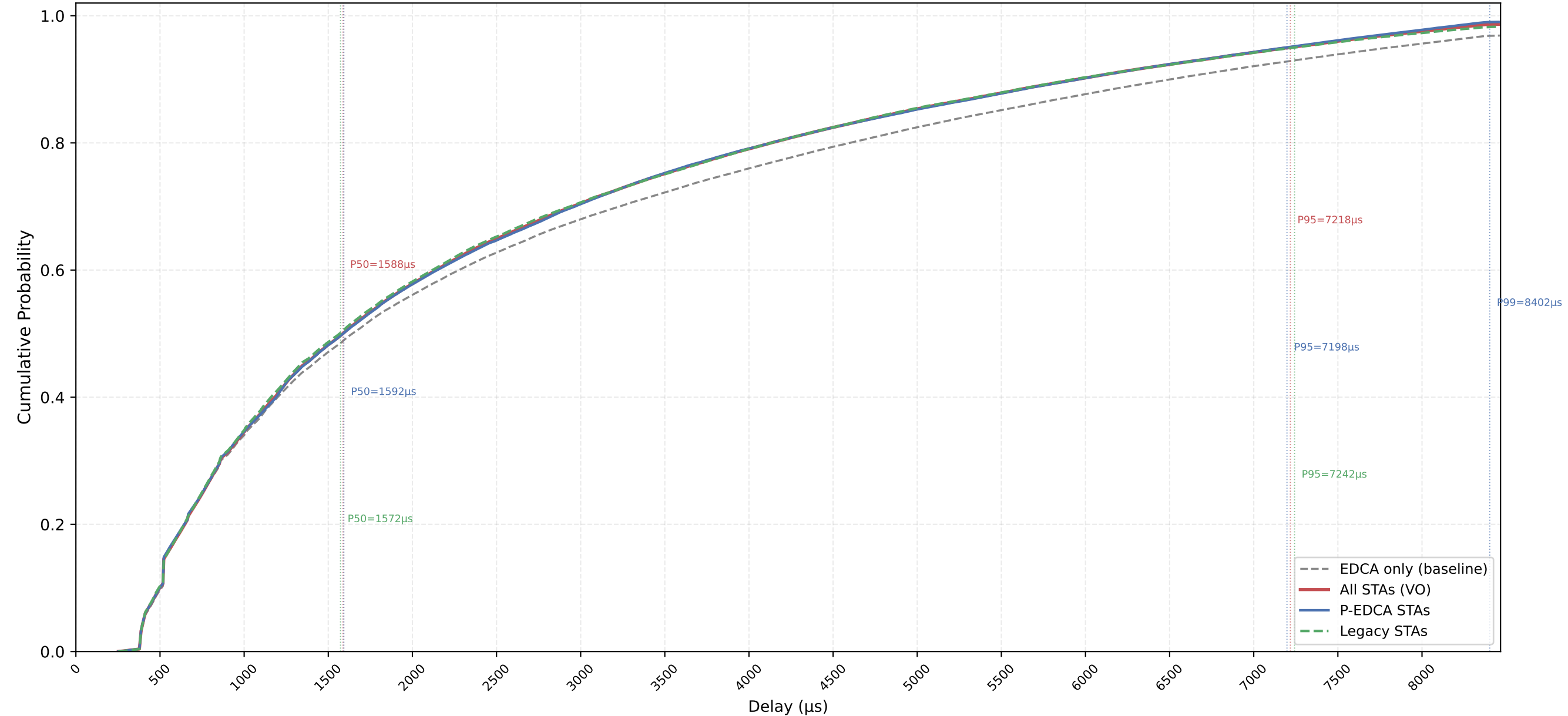
VO Delay CDF — P-EDCA / Legacy / All | CWds=0 × QSRC=4 × PSRC=2 nSta=30, nPedca=15/30, 1Mbps, avg of 10 runs
