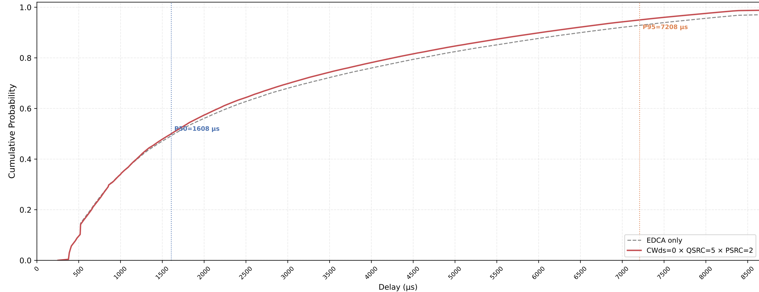
VO (all STAs) Delay CDF — CWds=0 × QSRC=5 × PSRC=2 nSta=30, nPedca=15, 1Mbps, avg of 10 runs
