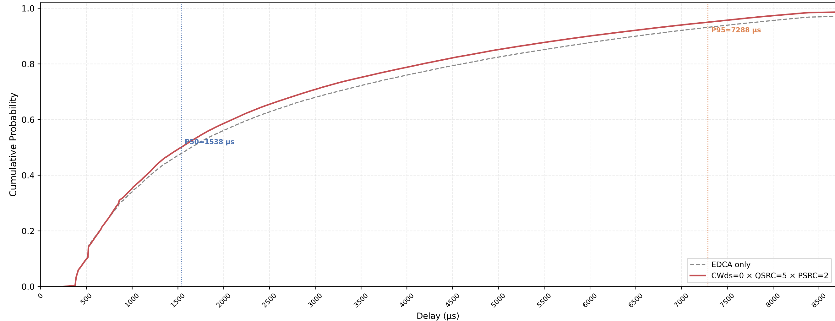
VO (all STAs) Delay CDF — CWds=0 × QSRC=5 × PSRC=2 nSta=30, nPedca=30, 1Mbps, avg of 10 runs
