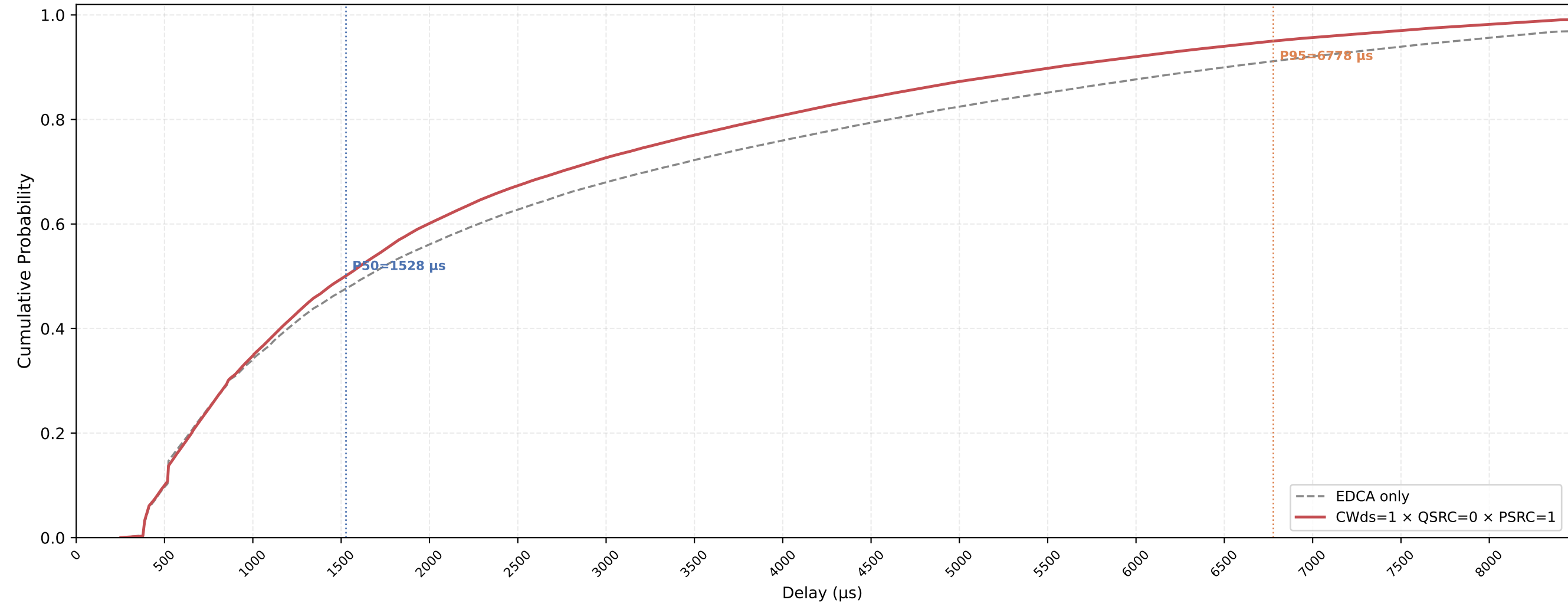
Legacy STA VO Delay CDF — CWds=1 × QSRC=0 × PSRC=1 nSta=30, nPedca=5, 1Mbps, avg of 10 runs
