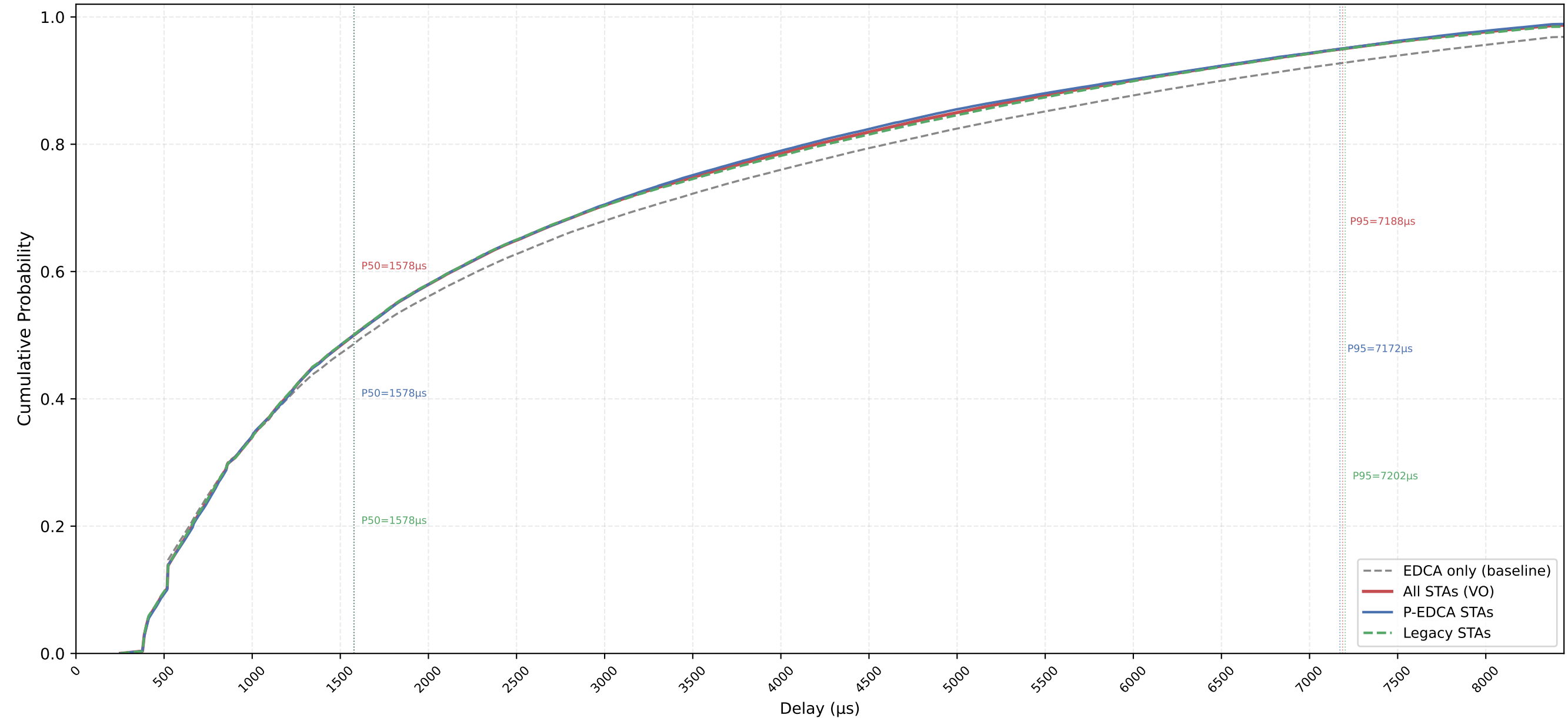
VO Delay CDF — P-EDCA / Legacy / All | CWds=1 × QSRC=5 × PSRC=3 nSta=30, nPedca=15/30, 1Mbps, avg of 10 runs
