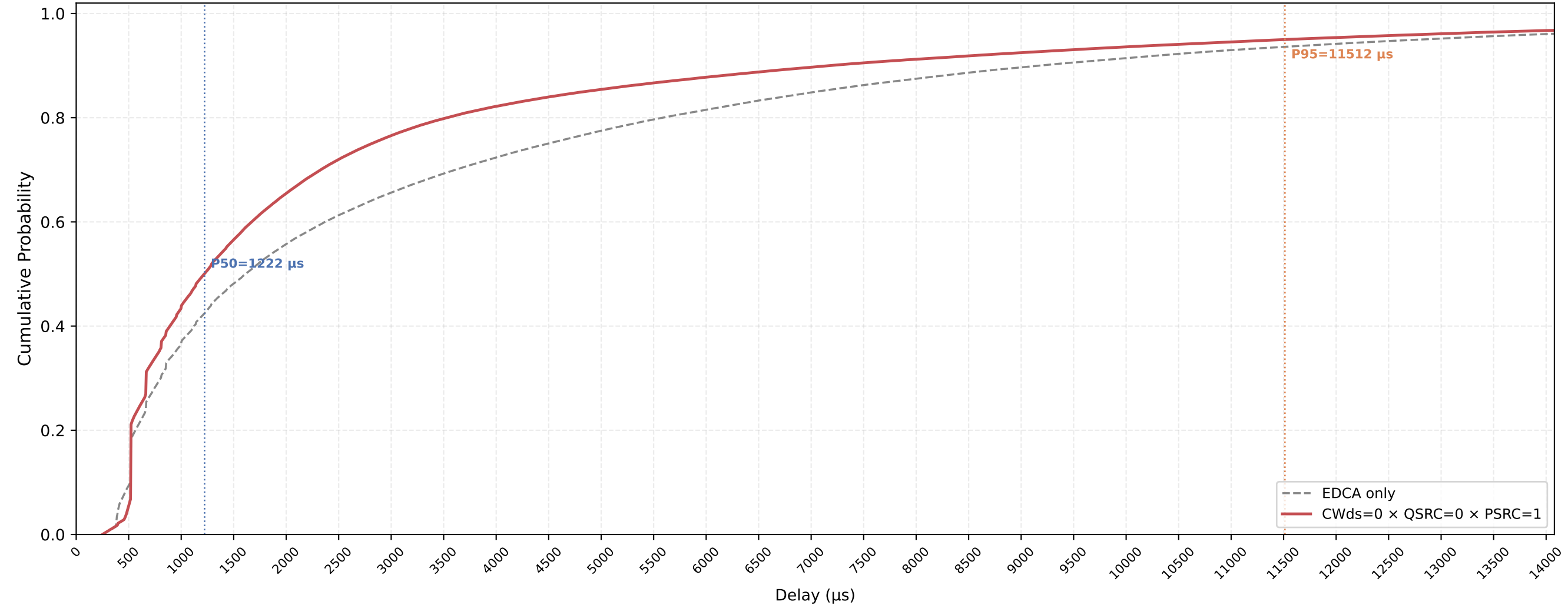
P-EDCA STA VO Delay CDF — CWds=0 × QSRC=0 × PSRC=1 nSta=30, nPedca=30, 1Mbps, avg of 10 runs
