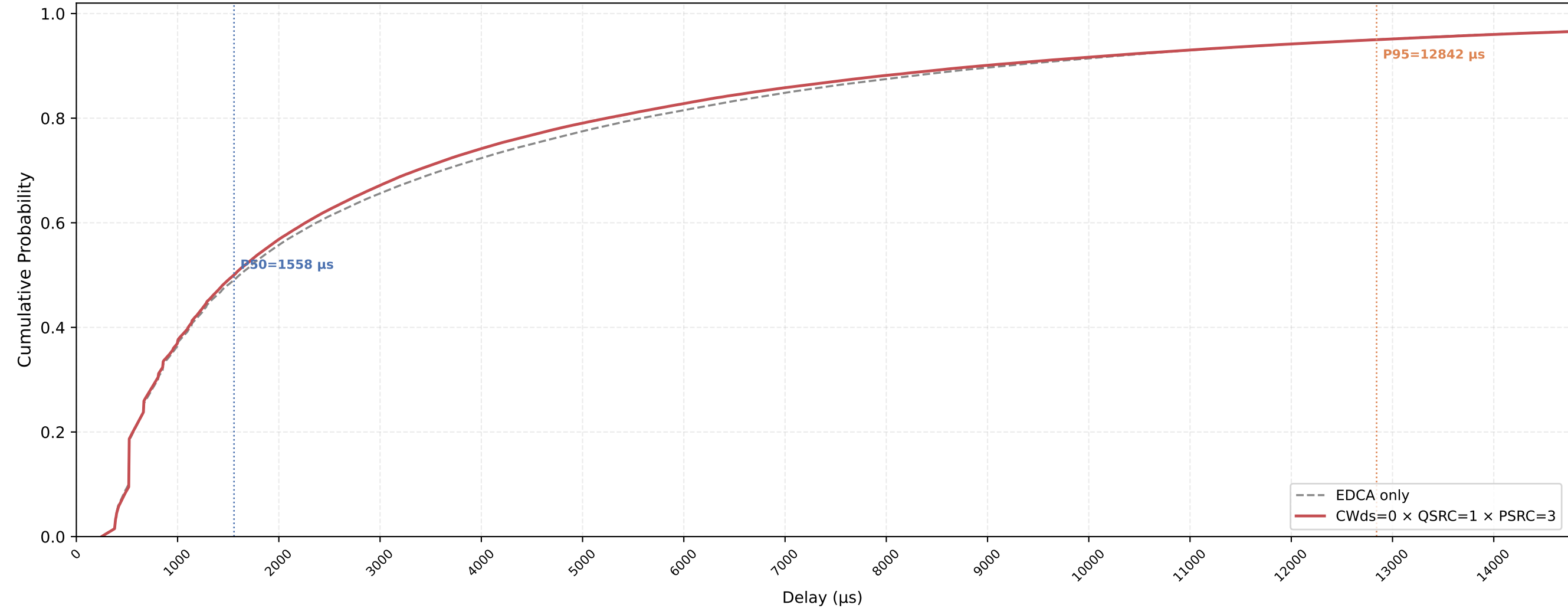
VO (all STAs) Delay CDF — CWds=0 × QSRC=1 × PSRC=3 nSta=30, nPedca=5, 1Mbps, avg of 10 runs
