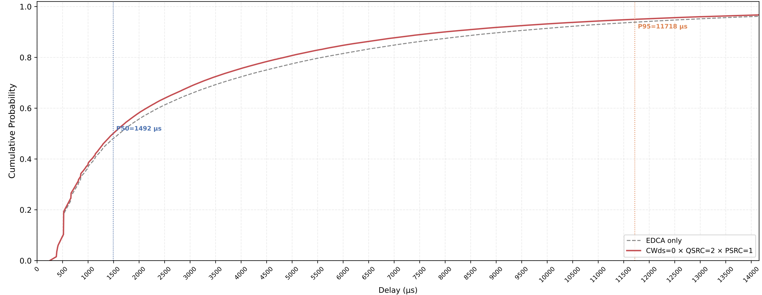
VO (all STAs) Delay CDF — CWds=0 × QSRC=2 × PSRC=1 nSta=30, nPedca=15, 1Mbps, avg of 10 runs
