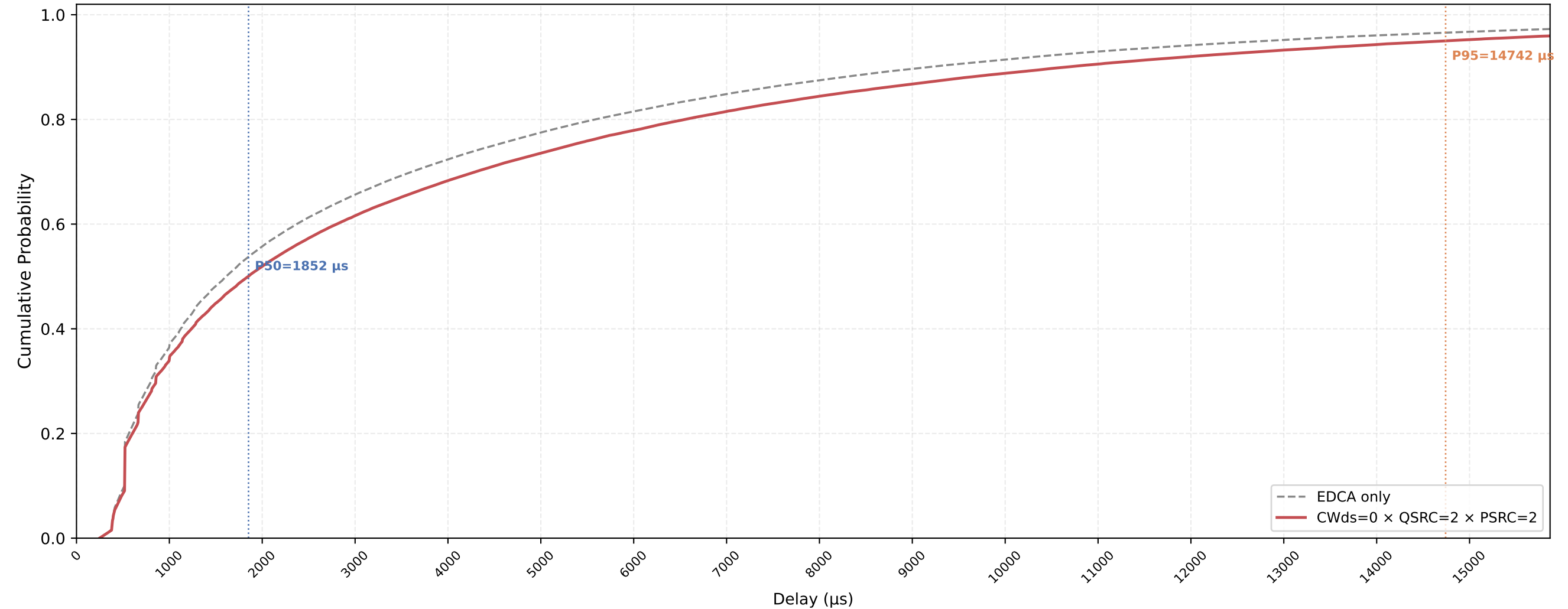
Legacy STA VO Delay CDF — CWds=0 × QSRC=2 × PSRC=2 nSta=30, nPedca=15, 1Mbps, avg of 10 runs
