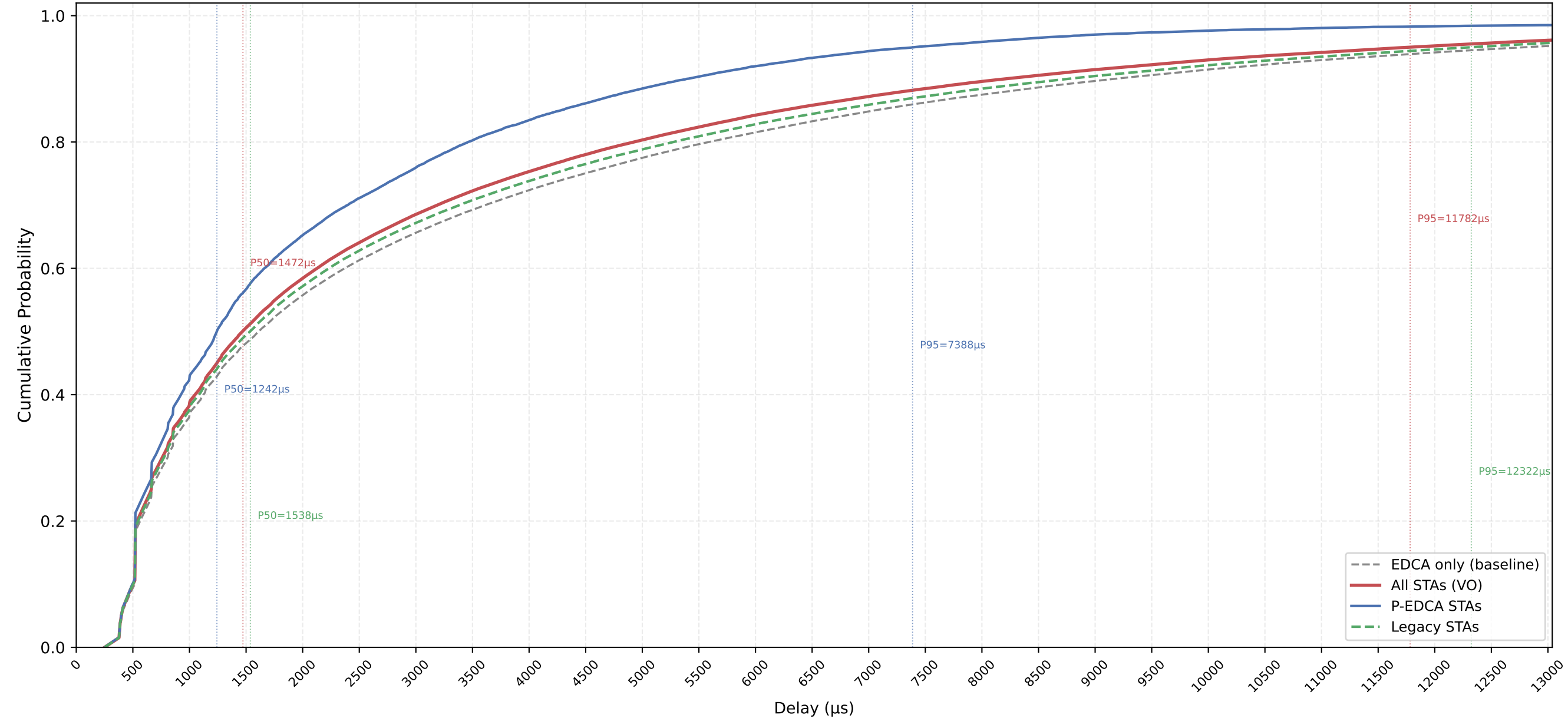
VO Delay CDF — P-EDCA / Legacy / All | CWds=0 × QSRC=2 × PSRC=3 nSta=30, nPedca=5/30, 1Mbps, avg of 10 runs
