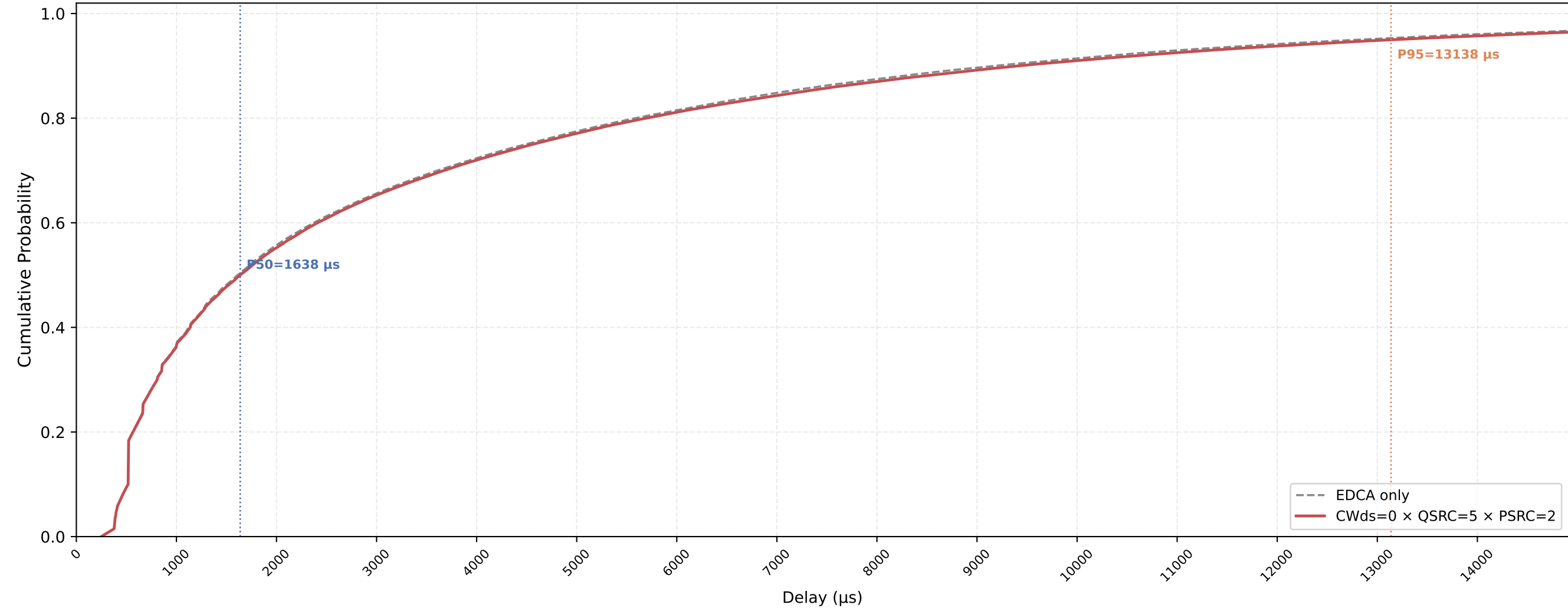
VO (all STAs) Delay CDF — CWds=0 × QSRC=5 × PSRC=2 nSta=30, nPedca=5, 1Mbps, avg of 10 runs
