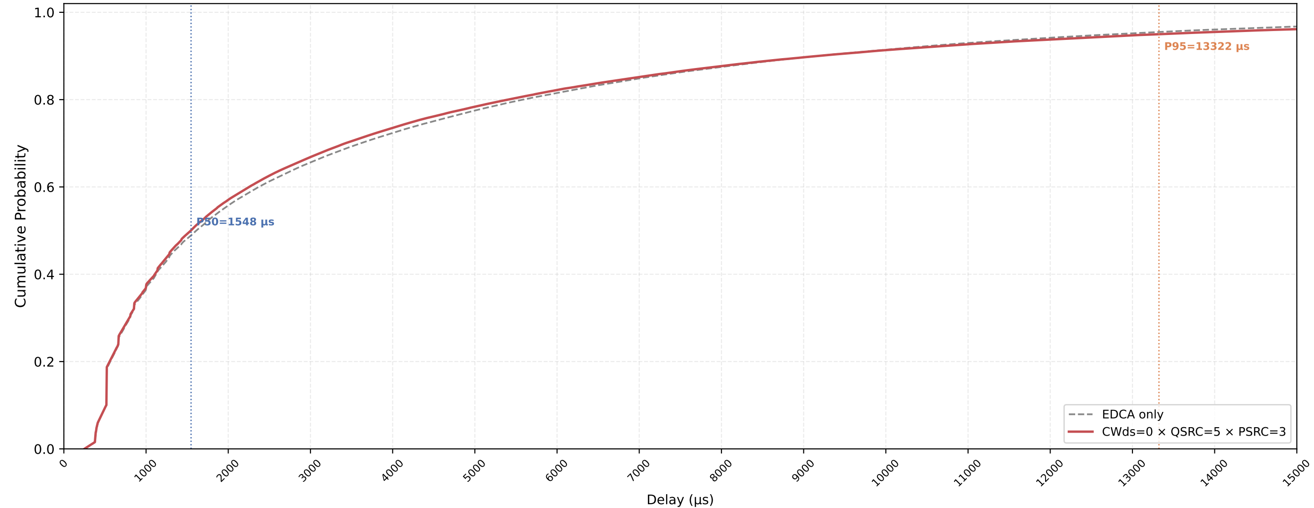
VO (all STAs) Delay CDF — CWds=0 × QSRC=5 × PSRC=3 nSta=30, nPedca=30, 1Mbps, avg of 10 runs
