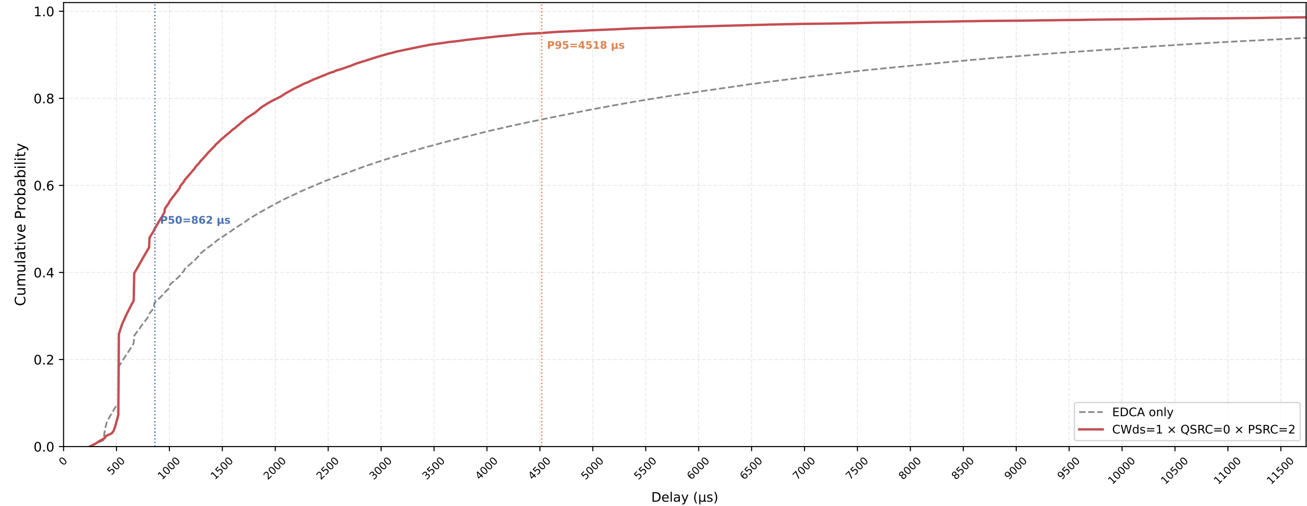
P-EDCA STA VO Delay CDF — CWds=1 × QSRC=0 × PSRC=2 nSta=30, nPedca=5, 1Mbps, avg of 10 runs
