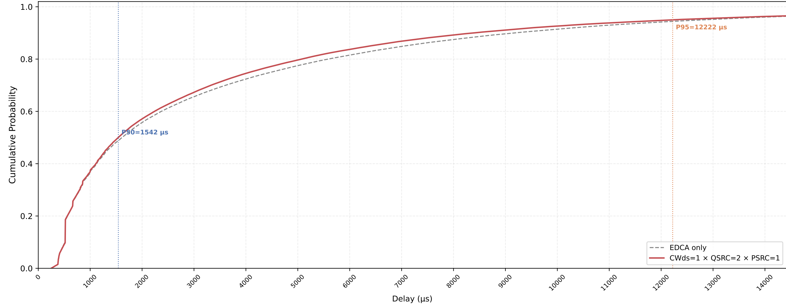
VO (all STAs) Delay CDF — CWds=1 × QSRC=2 × PSRC=1 nSta=30, nPedca=15, 1Mbps, avg of 10 runs
